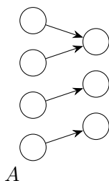
Surjection
