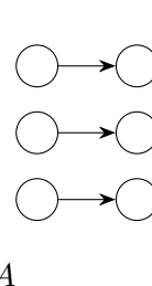
Bijection
