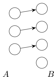
Injection
