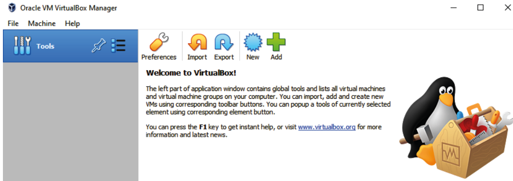
Figure 2.1 – VirtualBox interface
