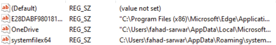
Figure 9.9 – Edited registry
