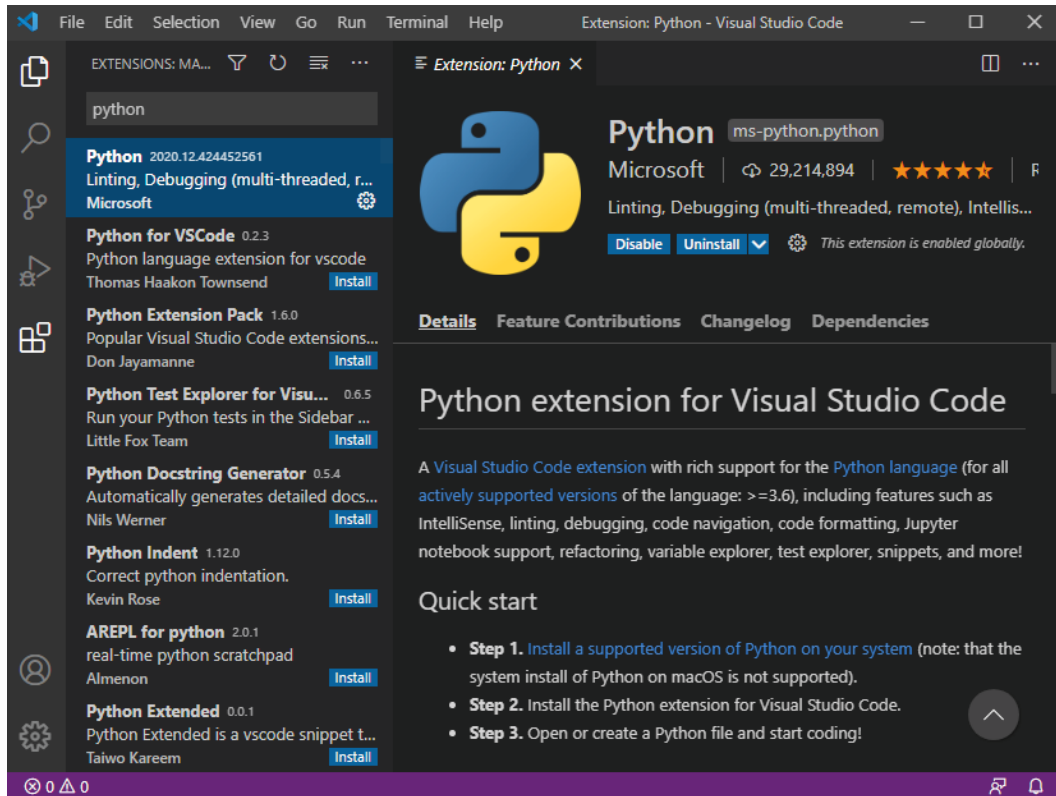
Figure 2.13 – Python extension
