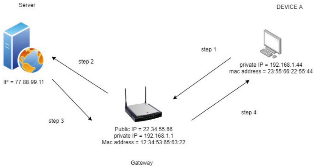
Figure 5.2 – Internet communication
