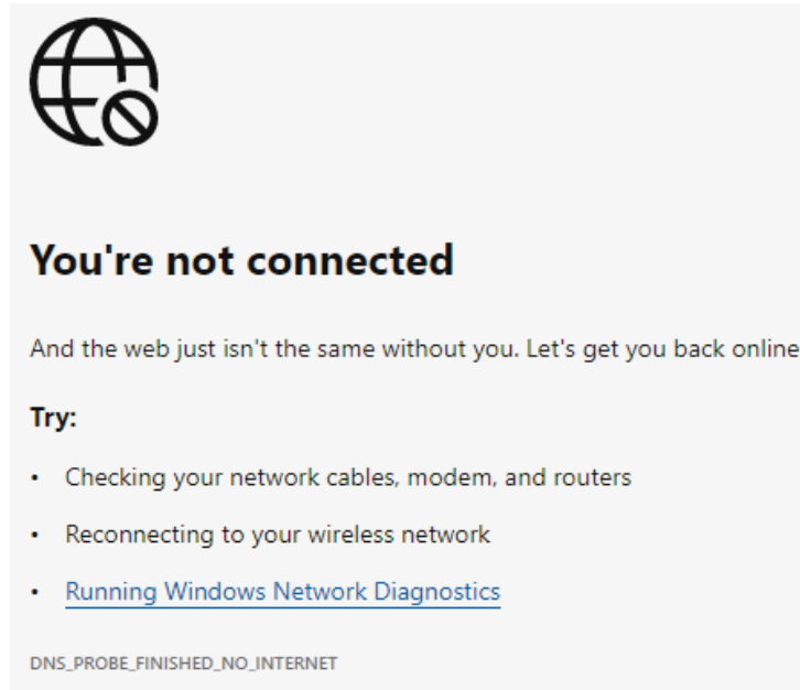
Figure 5.11 – No connection
