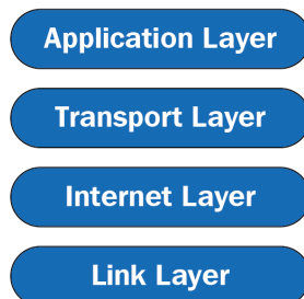
Figure 3.8 – TCP/IP stack
