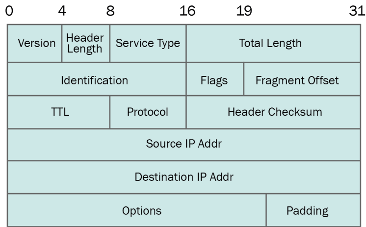
Figure 4.4 – IP header
