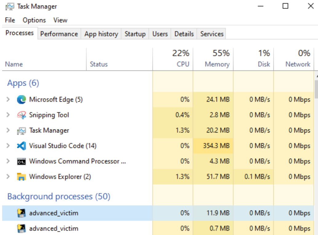
Figure 8.7 – Background process
