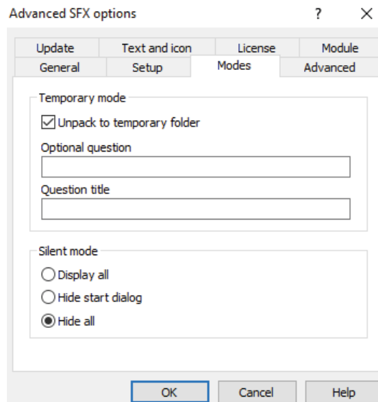
Figure 8.15 – SFX mode
