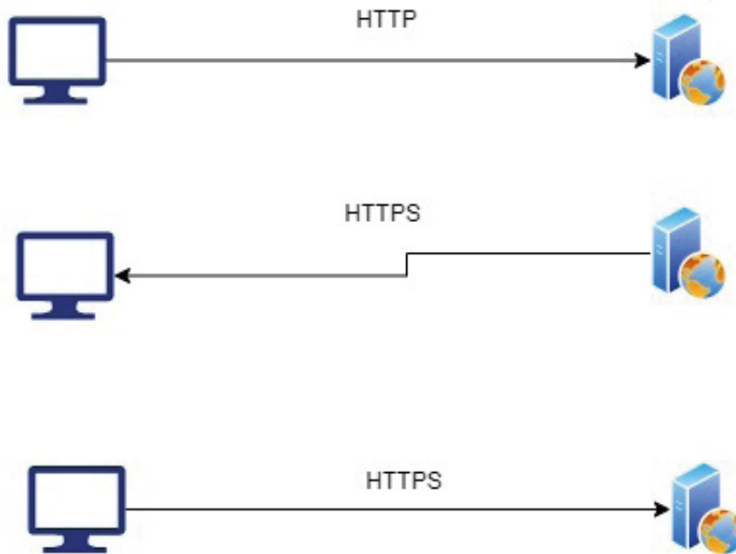
Figure 5.16 – HTTP cycle
