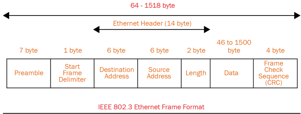
Figure 4.5 – Ethernet header
