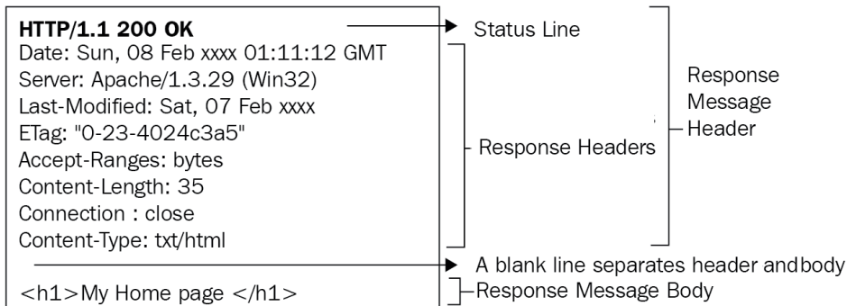
Figure 5.15 – HTTP reply
