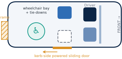
D · WAV (wheelchair-accessible variant)
