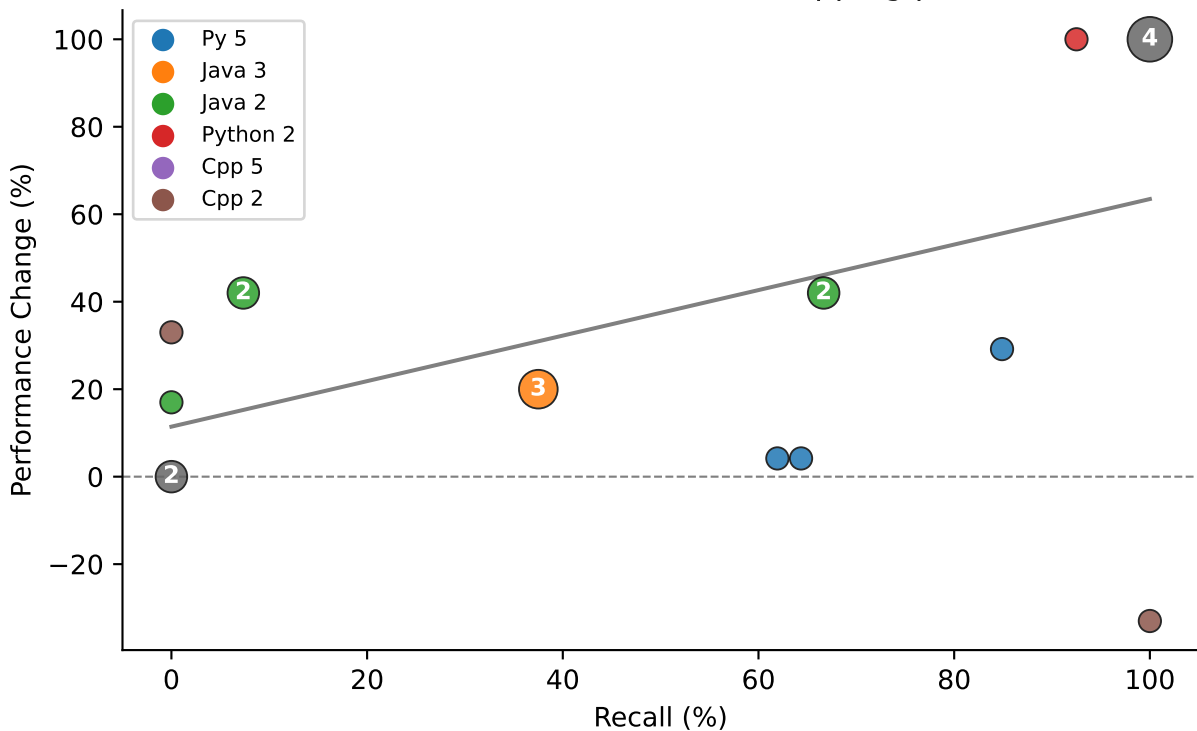
Recall vs Performance Change (%) (marker size + number = overlapping points)
