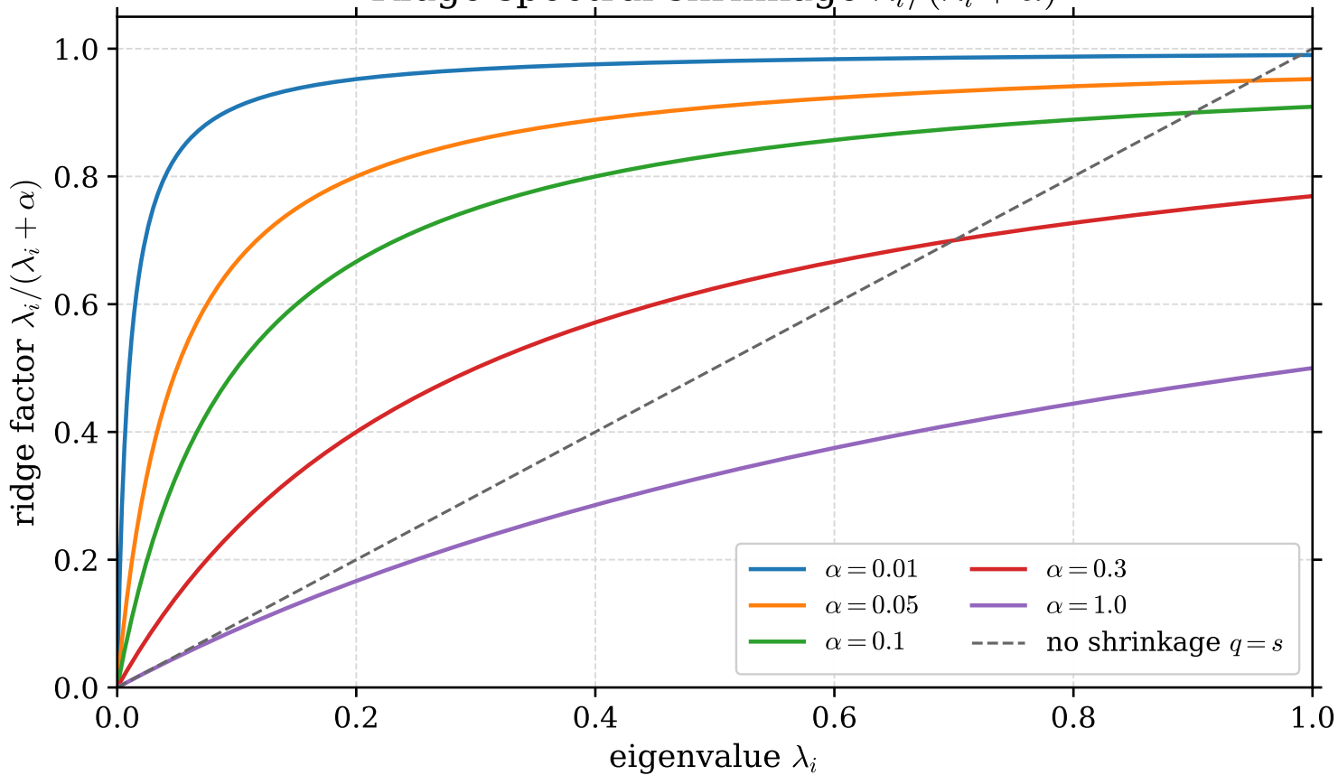
Ridge spectral shrinkage \lambda_i/(\lambda_i + \alpha)
