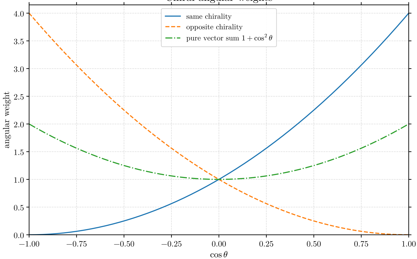
Chiral angular weights
