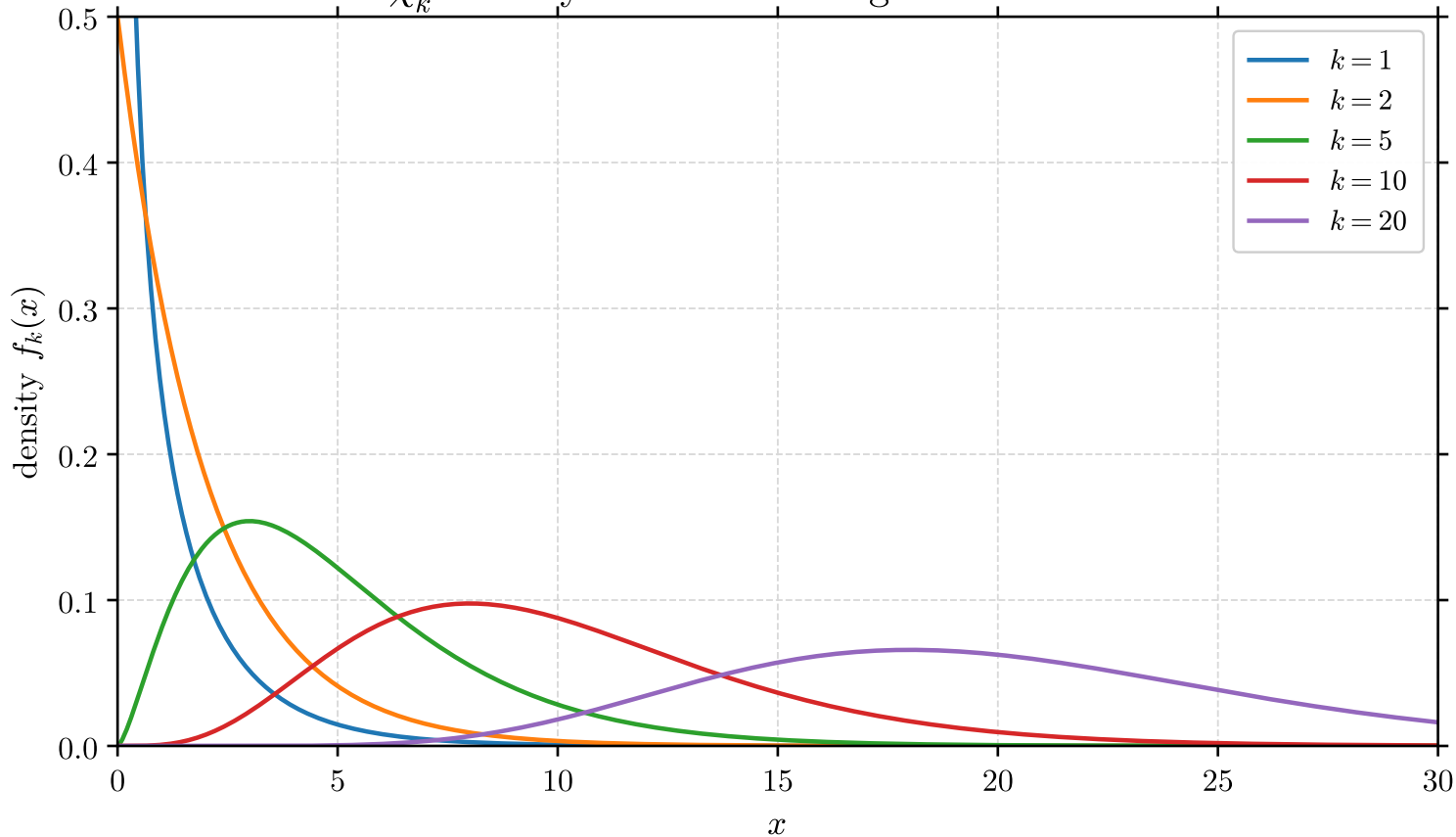
\chi_k^2 density for different degrees of freedom
