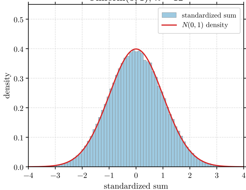
Uniform(0, 1), n = 12
