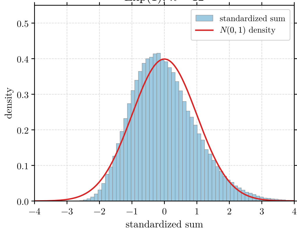
Exp(1), n = 12
