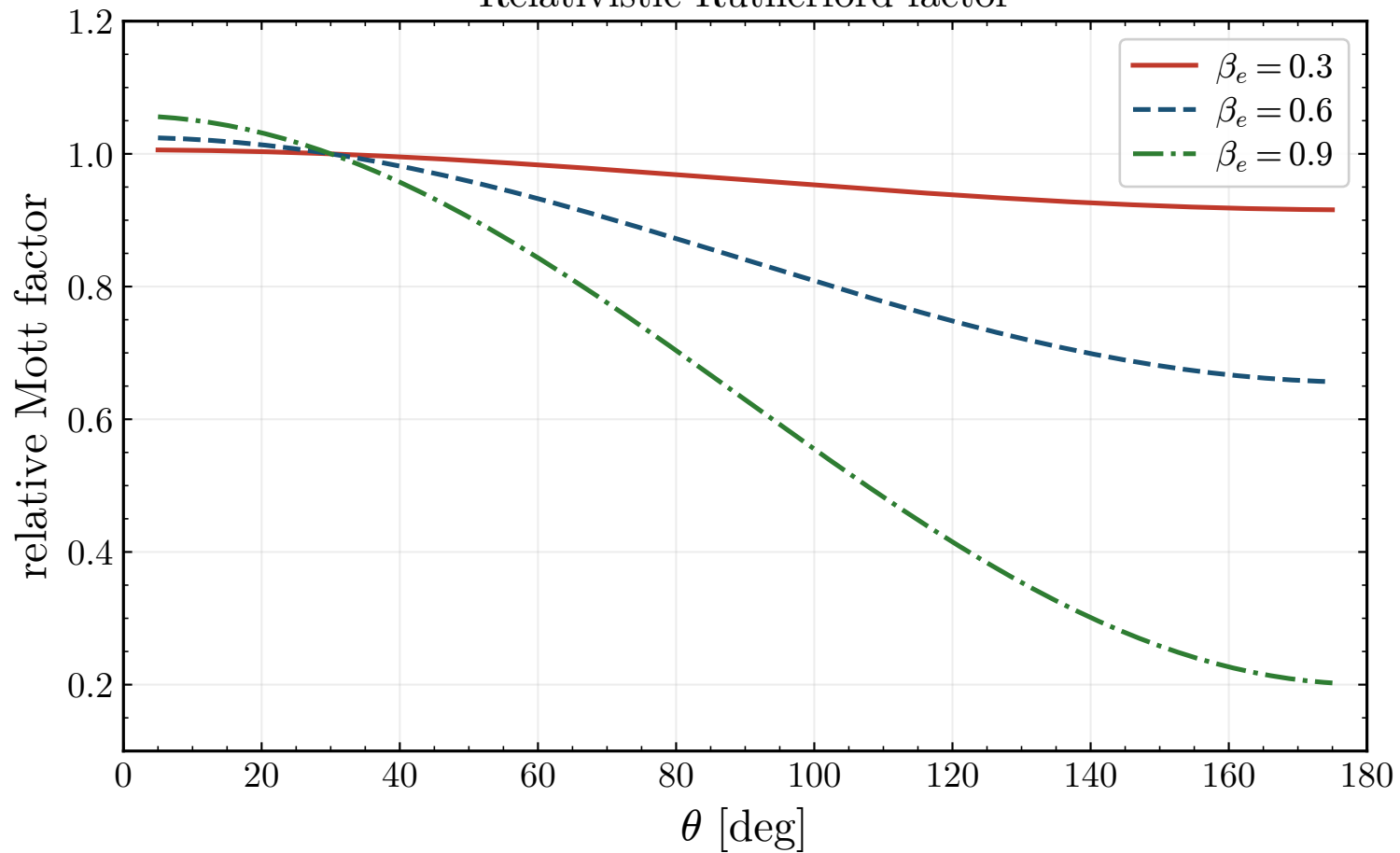
Relativistic Rutherford factor
