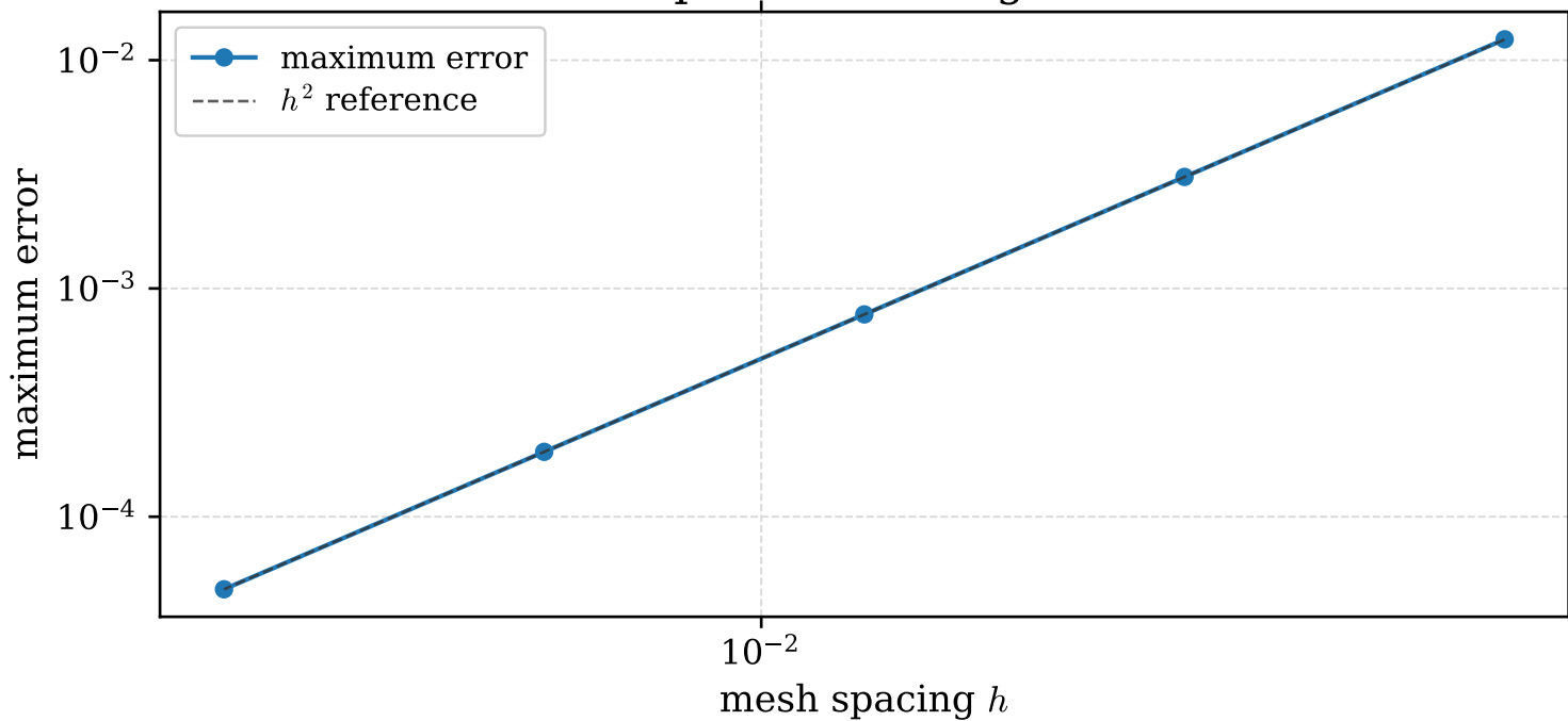
Trapezoid convergence
