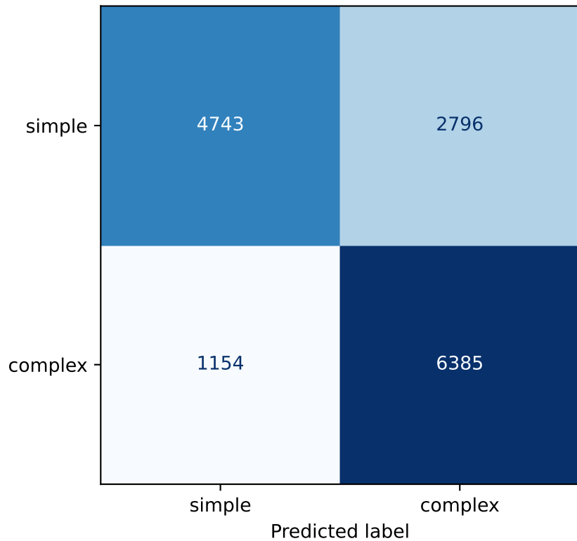
Logistic Regression
