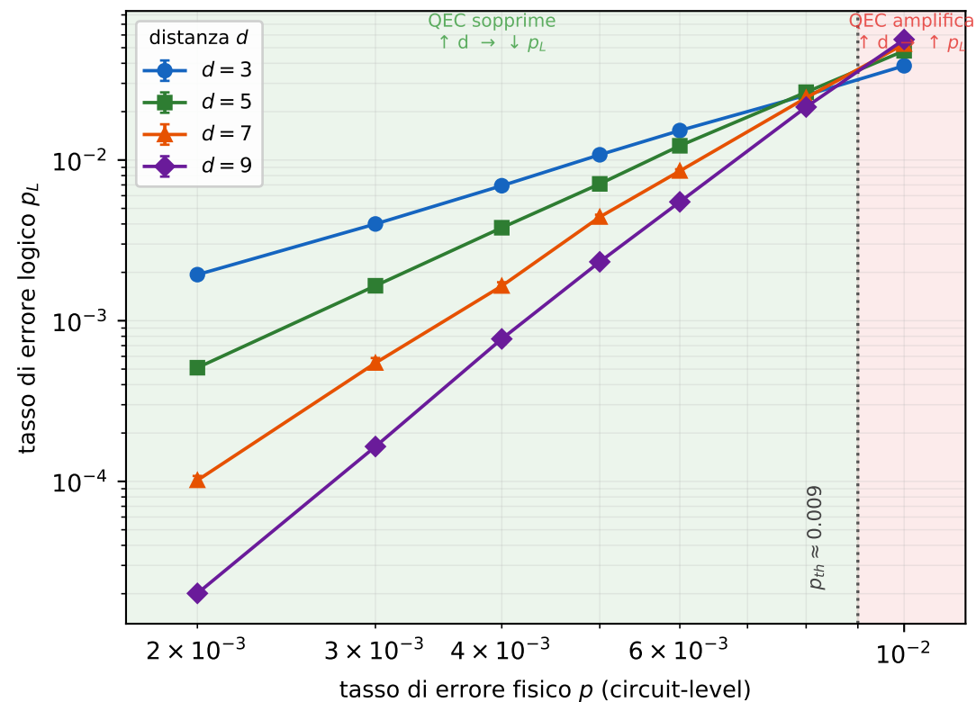
Surface code — base Z — decoder MWPM
