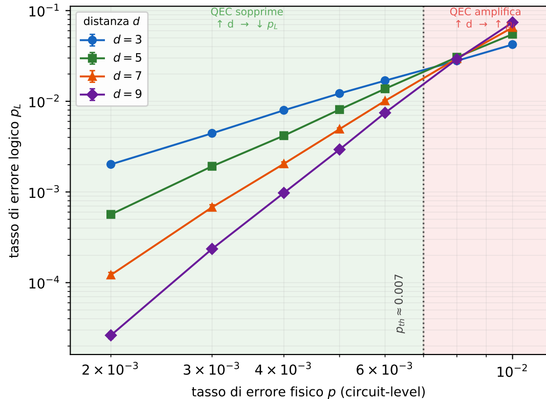
Surface code — base X — decoder MWPM
