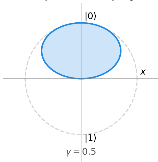
Amplitude damping
