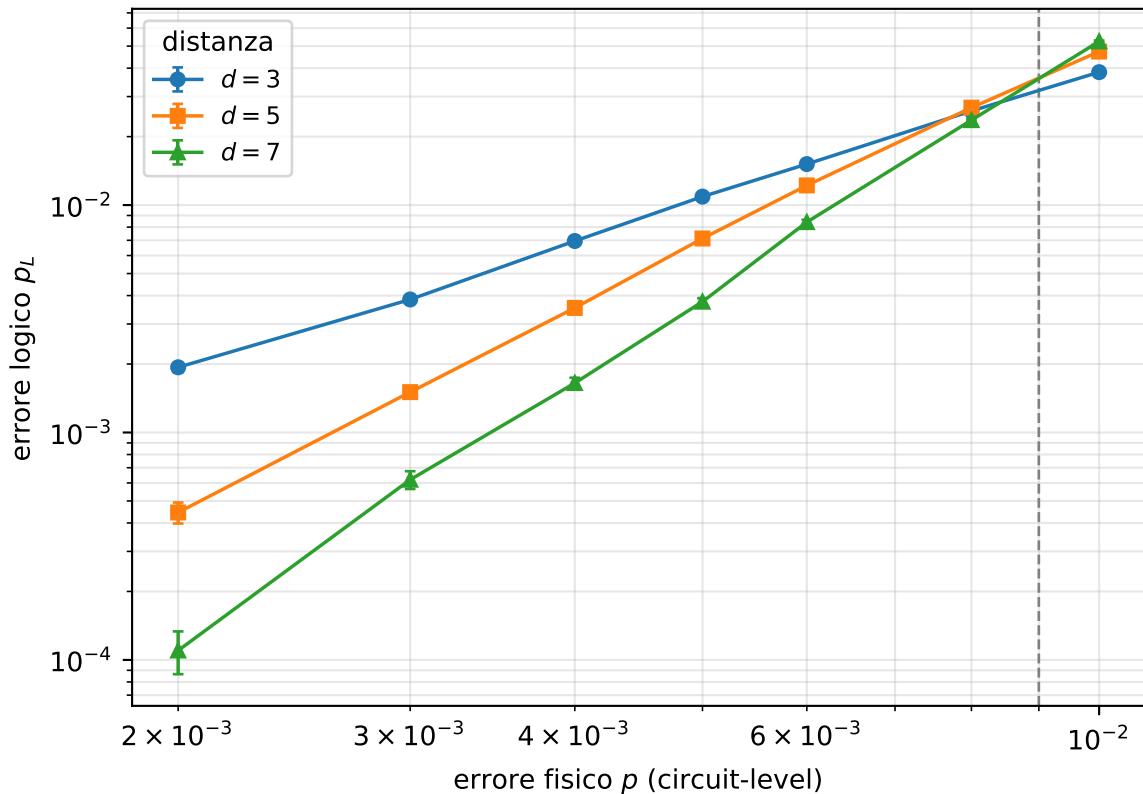
Surface code: comportamento a soglia (decoder MWPM)
