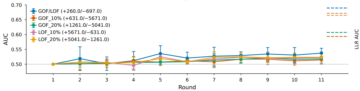
MC4R
