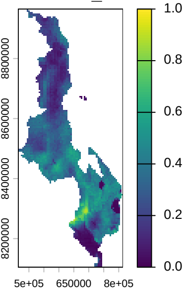
Model: 'all_cov'
