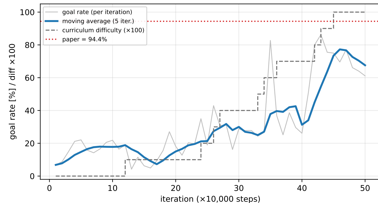
TD3 — no obstacles
