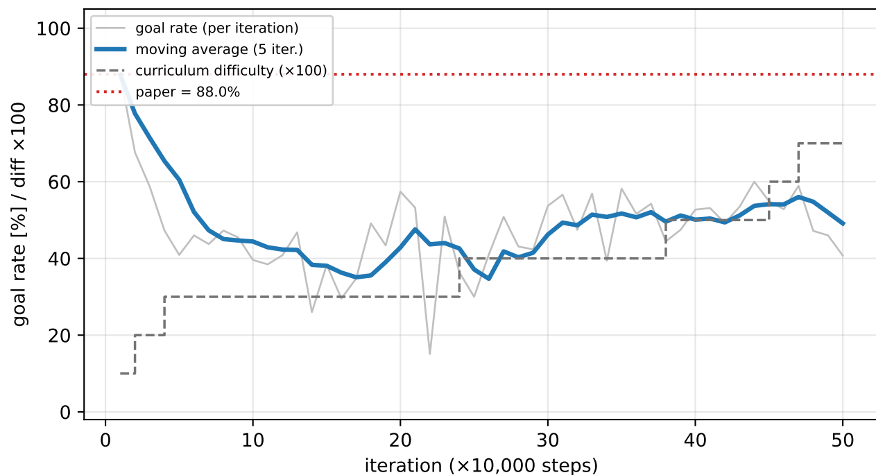
TD3 — with obstacles
