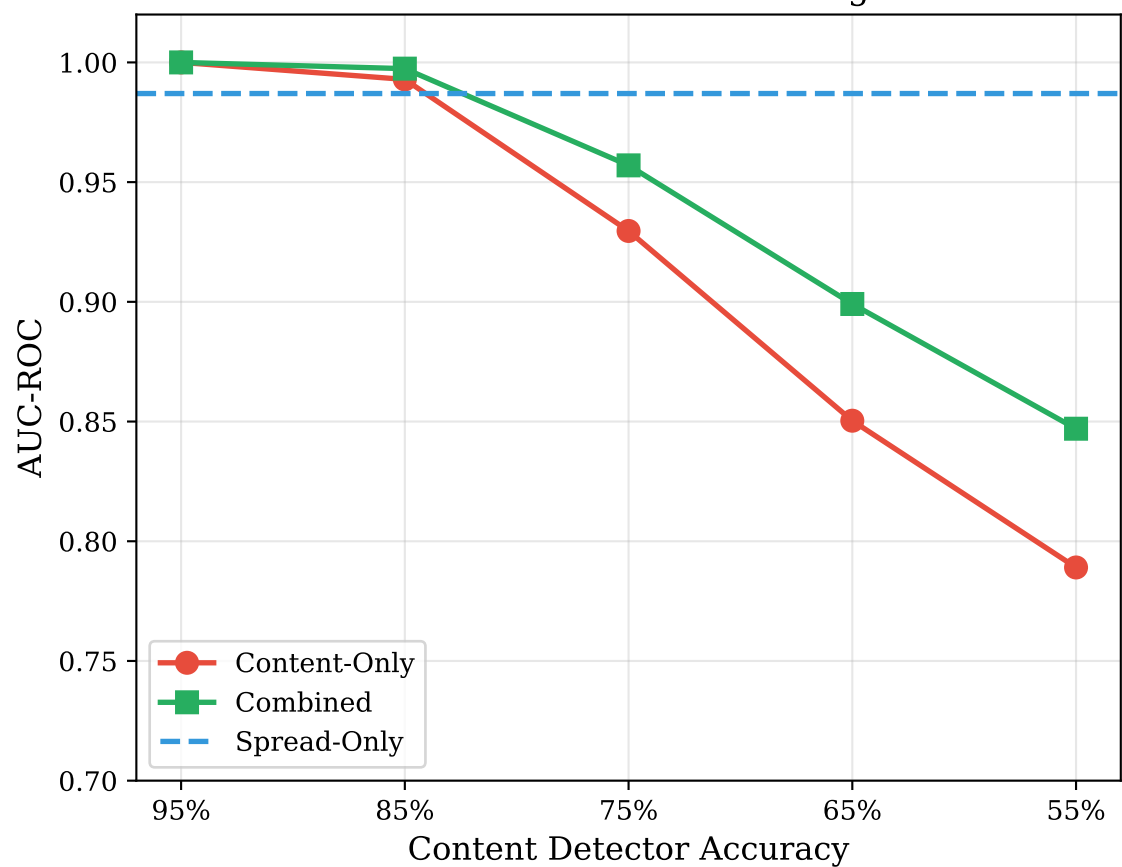
AUC-ROC vs. Content Detector Degradation
