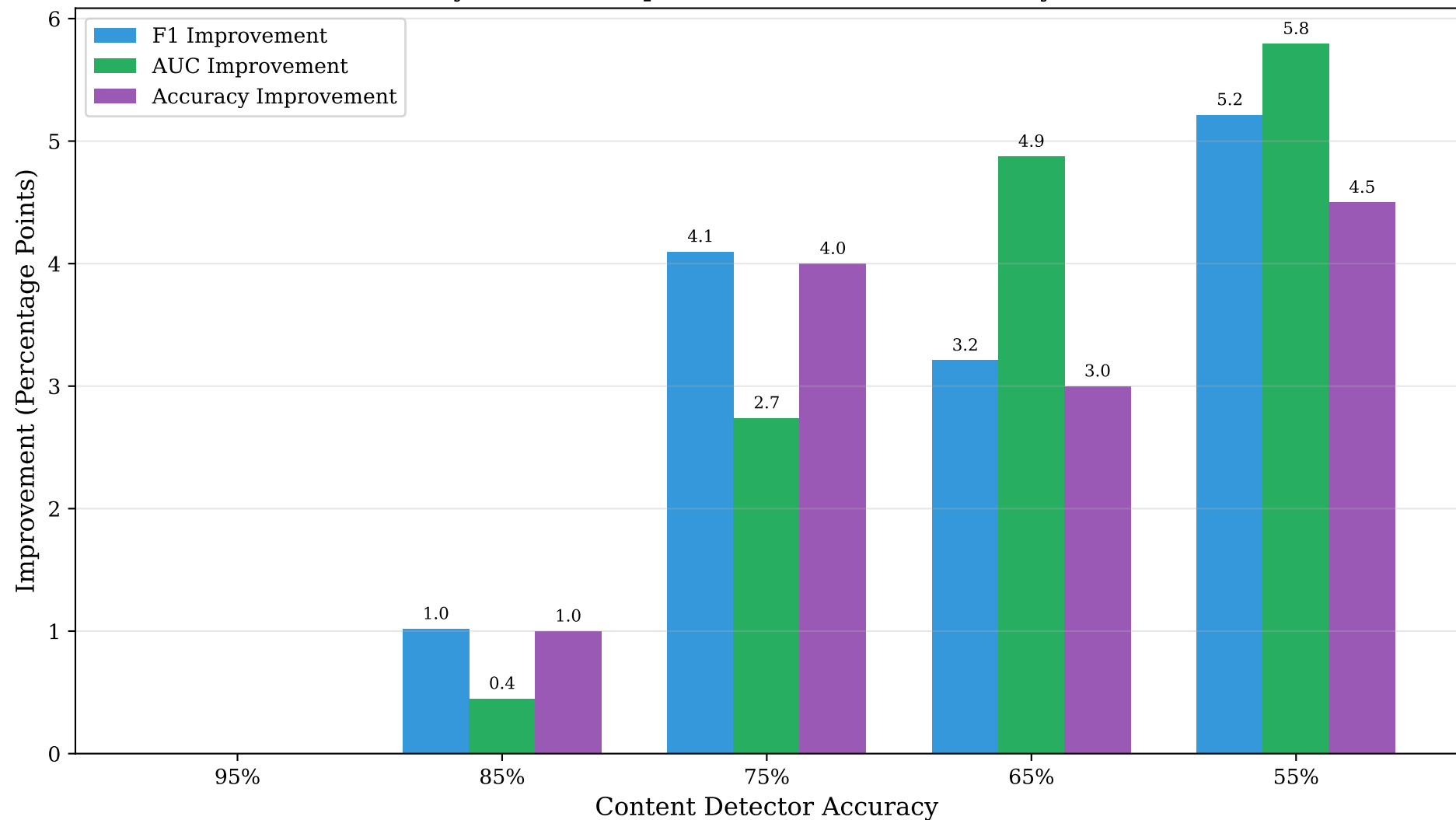
Multi-Layer Fusion Improvement Over Content-Only Detection
