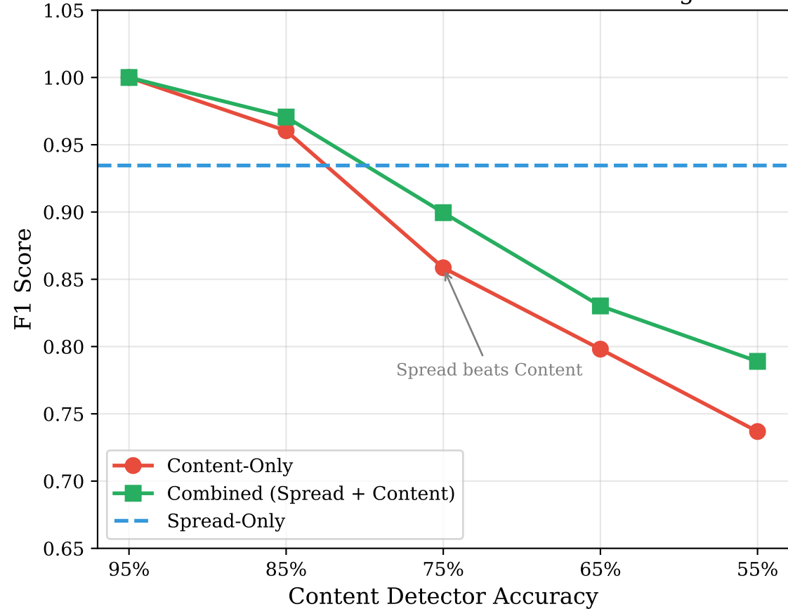
Detection Performance vs. Content Detector Degradation
