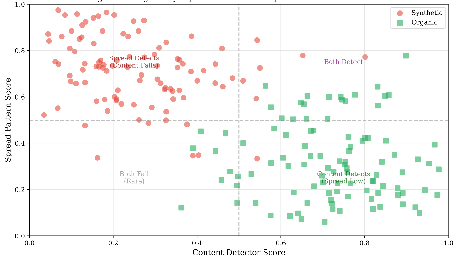
Signal Orthogonality: Spread Patterns Complement Content Detection
