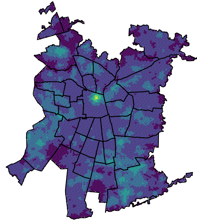
Pol-accessibility
