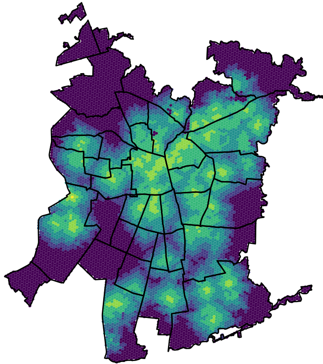
Pol-entropy
