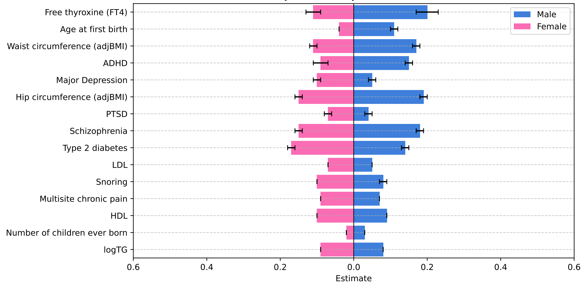
Heritability Estimates by Trait (Male vs. Female)
