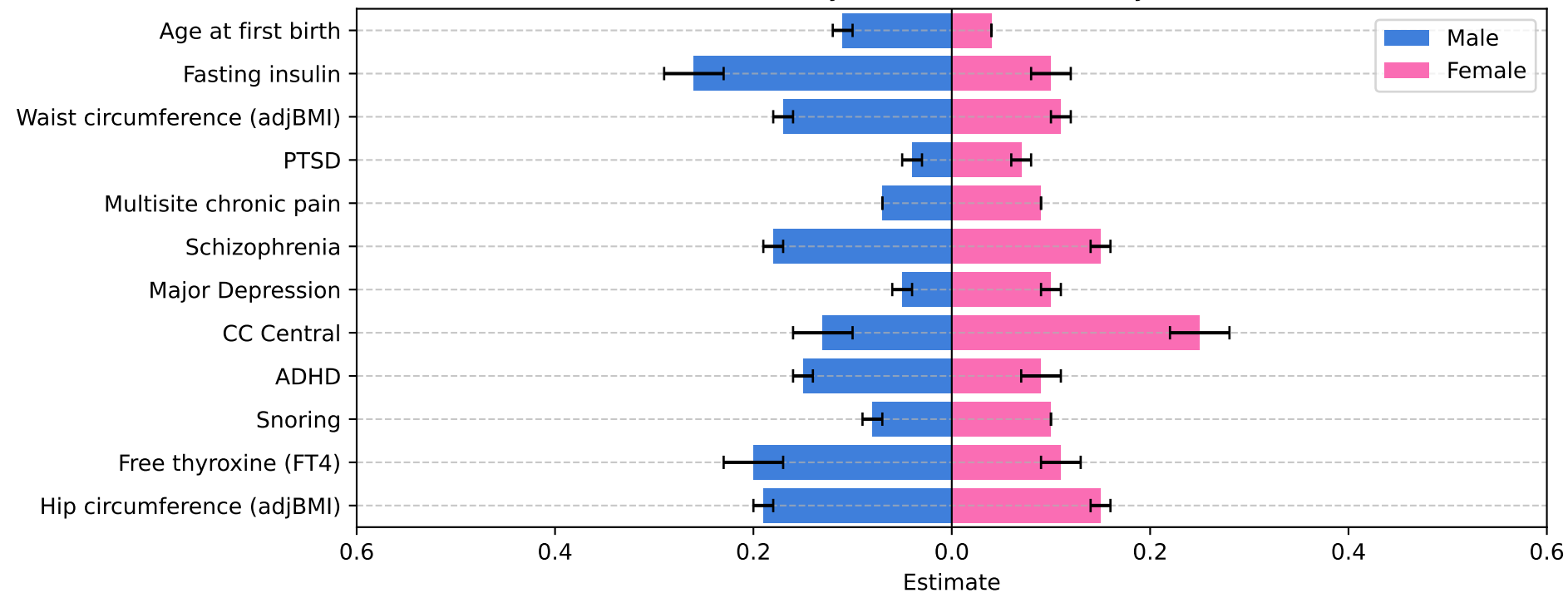
Heritability (SNP h 2 ) Estimates by Sex
