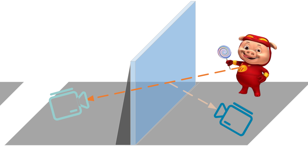
(c) Mirror-3DGS
