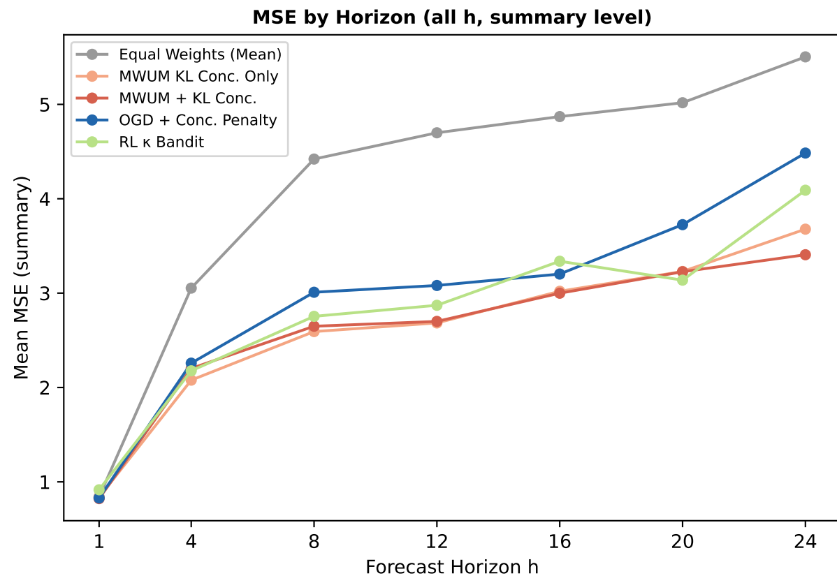
Figure 5: Horizon Effect — Concentration Penalties Gain More at Longer Horizons (H3)
