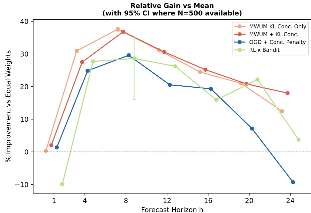
Figure 5: Horizon Effect — Concentration Penalties Gain More at Longer Horizons (H3)
