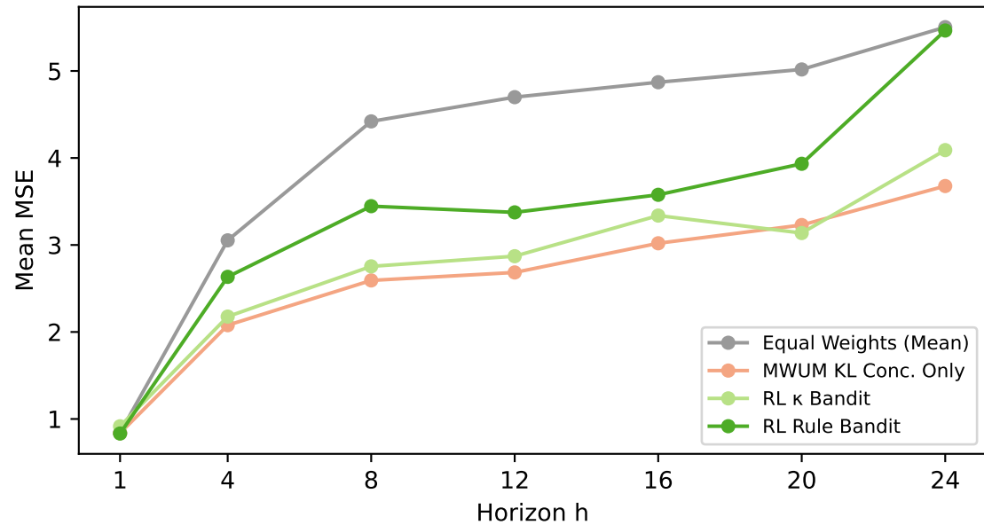
RL Bandits vs Benchmarks (MSE by Horizon)
