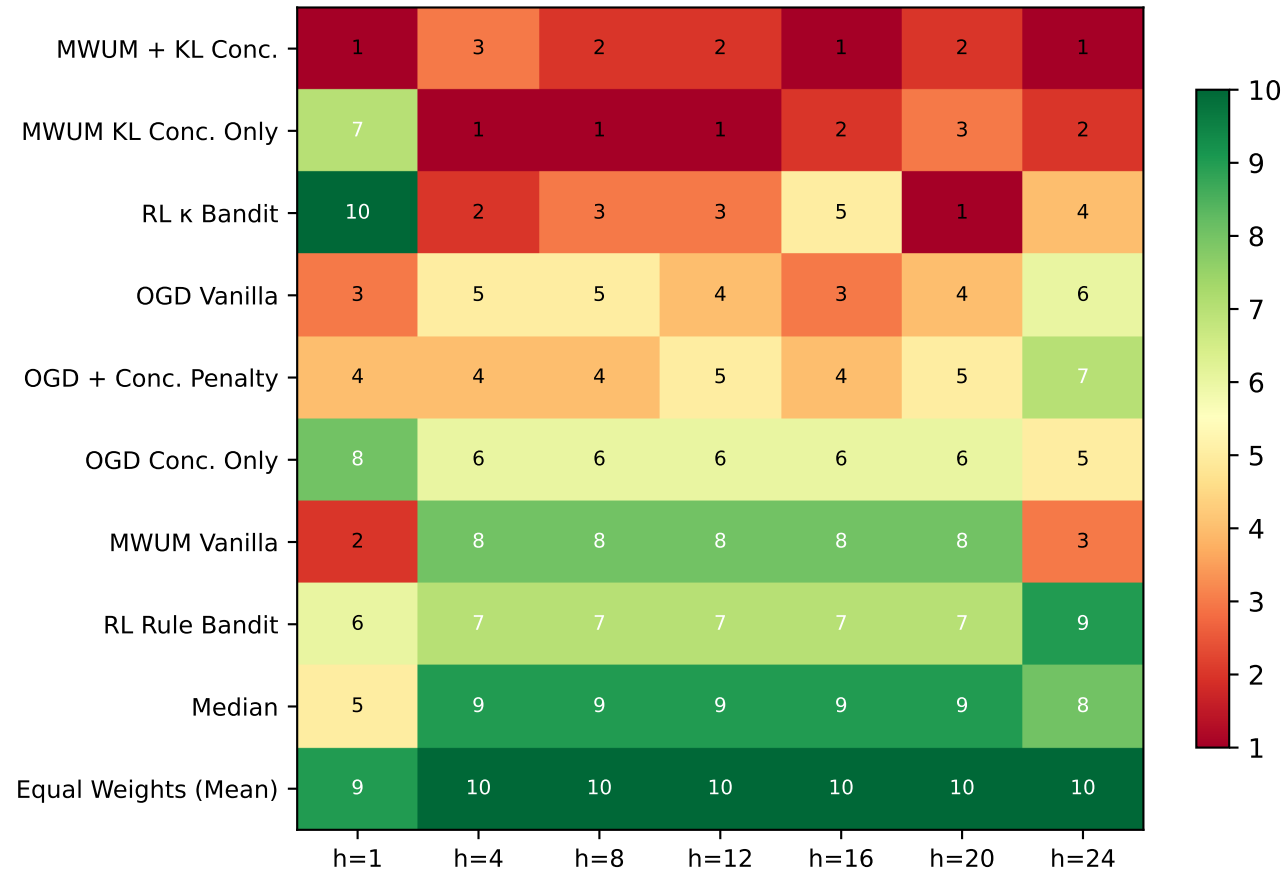
Figure 2: Rank (1 = best)
