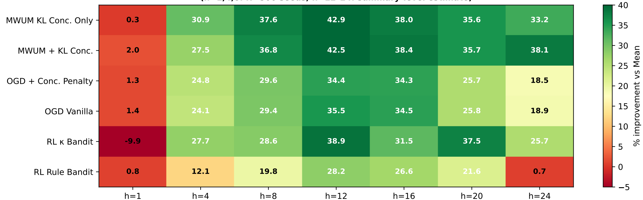
Figure 8: % Improvement over Equal-Weight Benchmark (MSE) ( h=1,4,8 : N=500 seeds; h=12-24 : summary-level estimate)
