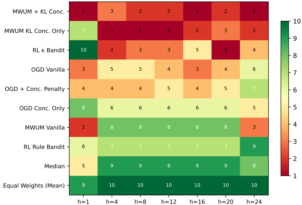
Figure 2: Rank (1 = best)
