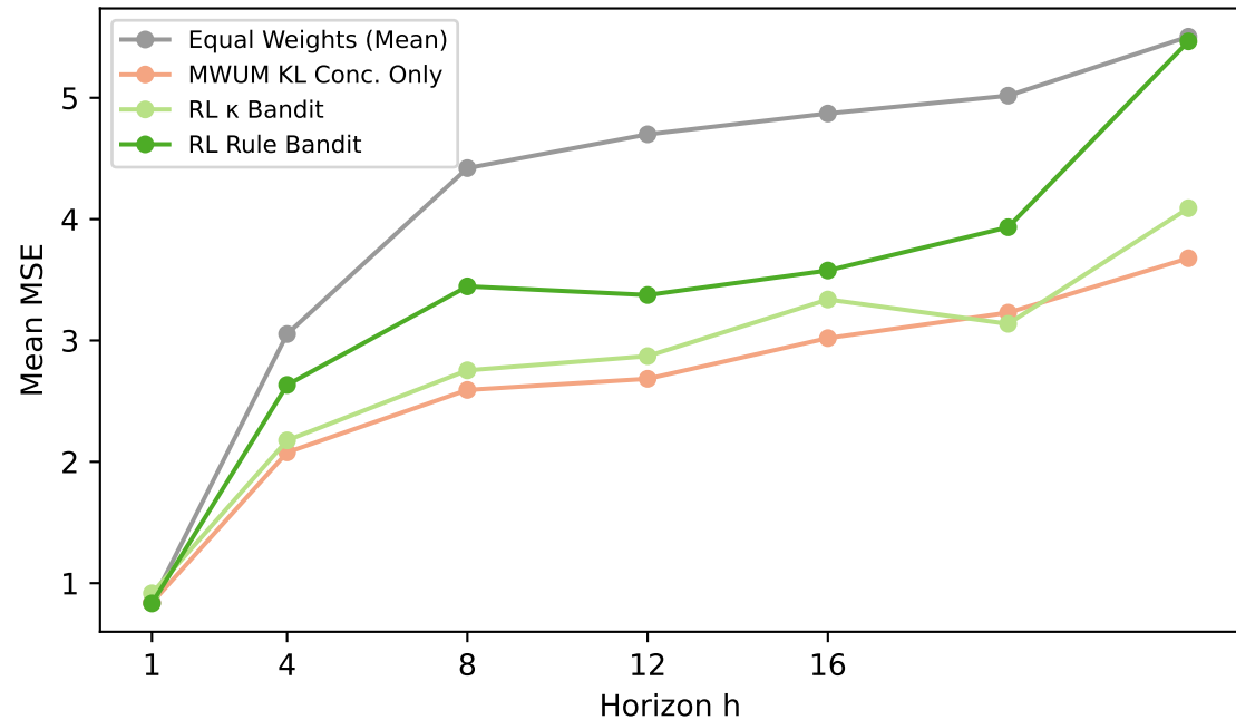
RL Bandits vs Benchmarks (MSE by Horizon)
