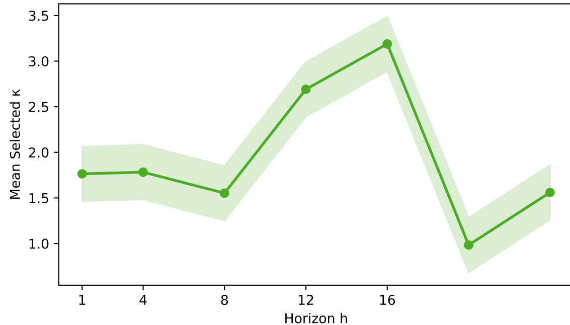
Learned Concentration Strength by Horizon (RL \kappa Bandit)
