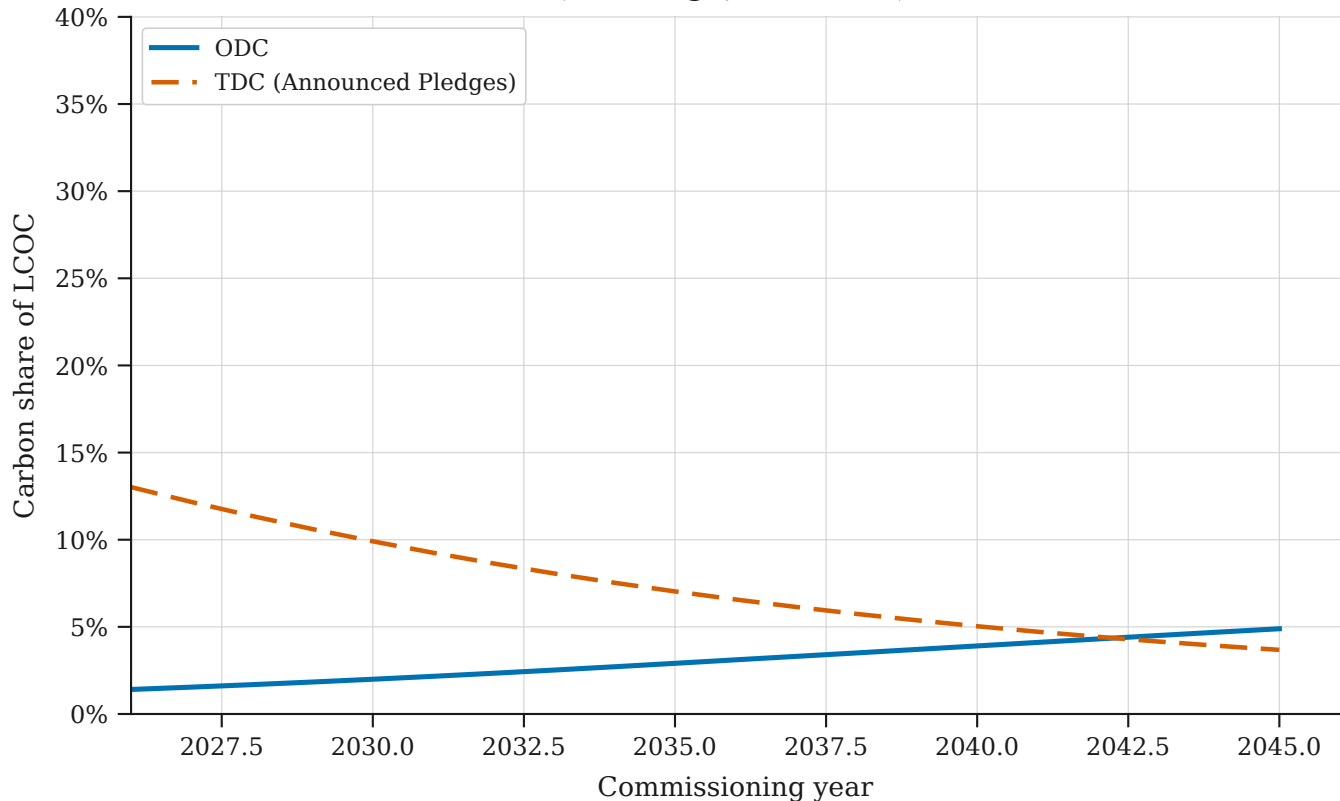
Carbon as a share of LCOC (carbon @ $185/tCO 2 e)
