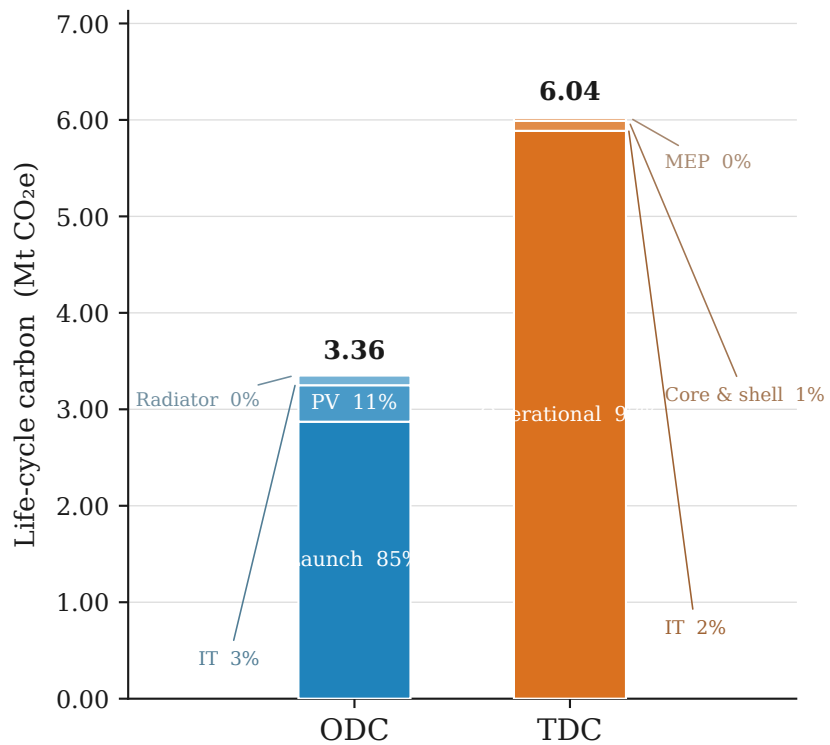
(B) Carbon composition | TDC/ODC = 1.8×
