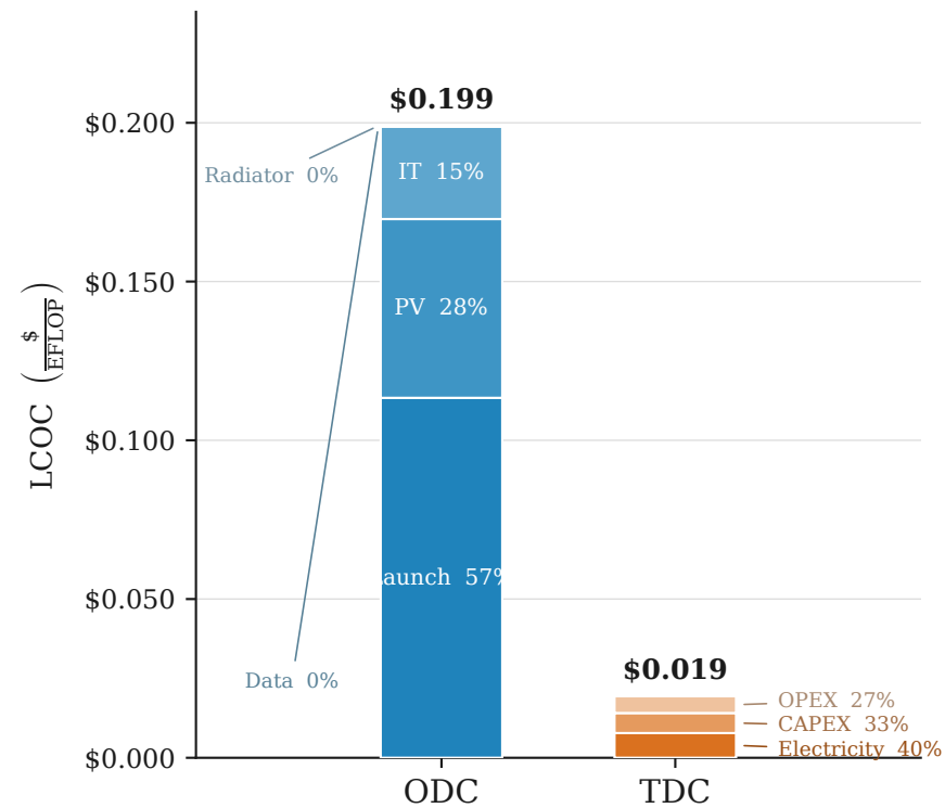
(A) Cost composition | ODC/TDC = 10.3×
