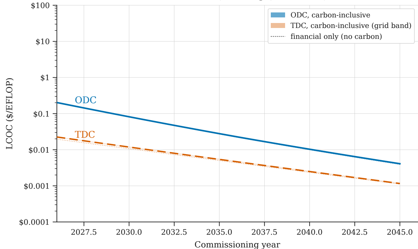
Carbon-inclusive LCOC over time (carbon @ $185/tCO 2 e)
