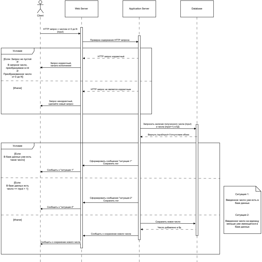
Sequence diagram
