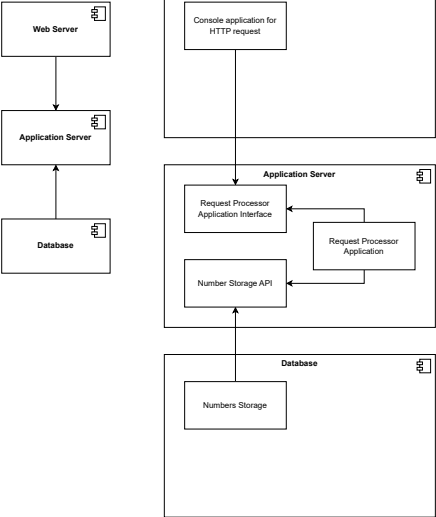
Component diagram
