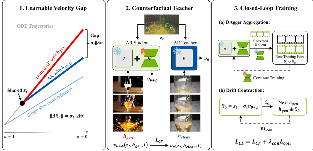
Figure 2: Overview of Clean Forcing. \theta denotes the frozen base weights and \phi the LoRA corrector r_\phi . (1) At the shared noisy state z_t , \Delta v := v_\theta(z_t, h_{\text{clean}}, t) - v_\theta(z_t, h_{\text{gen}}, t) is the history-induced velocity gap. The corresponding one-step clean-latent predictions differ by \sigma_t \|\Delta v\| , contributing to drift over successive chunks. (2) The LoRA student conditions on h_{\text{gen}} and matches the frozen teacher’s prediction under h_{\text{clean}} ( \mathcal{L}_{\text{CF}} ). (3a) We generate new training pairs D_\phi with the corrector active and continue training on D_0 \cup D_\phi , where D_0 contains pairs from uncorrected rollouts. (3b) \mathcal{L}_{\text{con}} backpropagates the next chunk’s error through the undetached prediction \hat{x}_0 .
