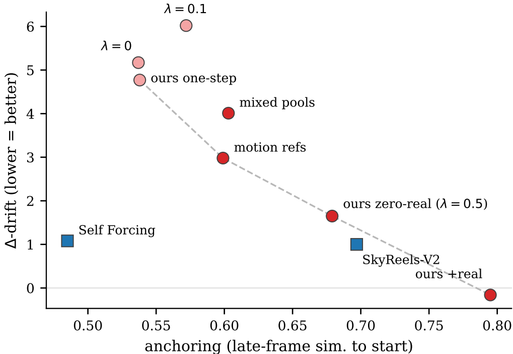
Figure 5: Drift reduction and scene progression. Anchoring is the DINO (Caron et al., 2021) similarity between the opening and final fifths of a video; higher values indicate less progression. Hollow circles show Clean Forcing variants, filled circles its reported zero-real and +real configurations, and squares other systems. Across Clean Forcing settings, lower \Delta -drift generally coincides with higher anchoring. Self Forcing, trained on over 10^5 clips, achieves low drift with less anchoring.
