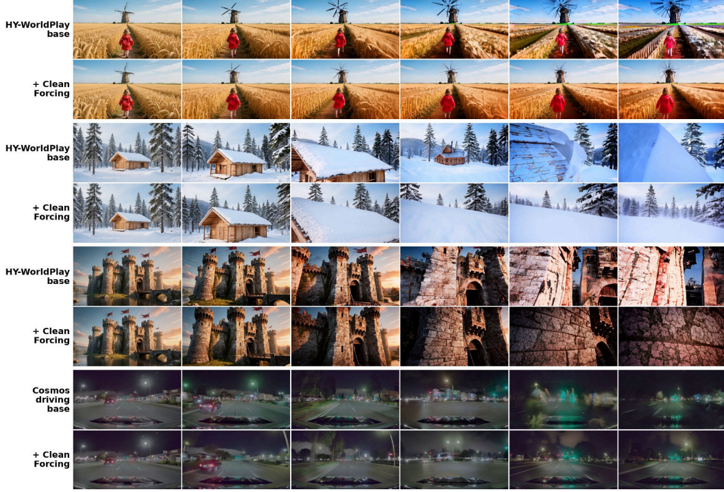
Figure 11: Correction on other autoregressive world models. Six evenly spaced frames from three HY-WorldPlay rollouts ( \sim 24 s) and one Cosmos-based driving rollout ( \sim 80 s). Each base and corrected pair shares its prompt, conditioning, and seed. We use strengths of 0.5\alpha^*(t) for HY-WorldPlay and 0.25\alpha^*(t) for the driving model. The corrected rollouts better retain color, detail, and scene structure as the base rollouts degrade.
