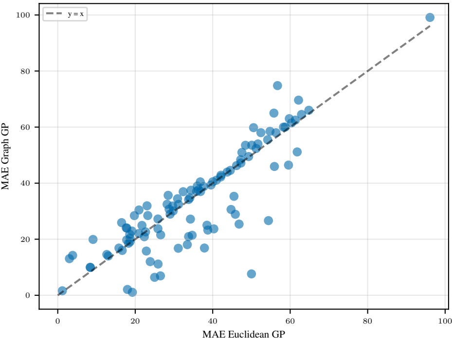
MAE Comparison
