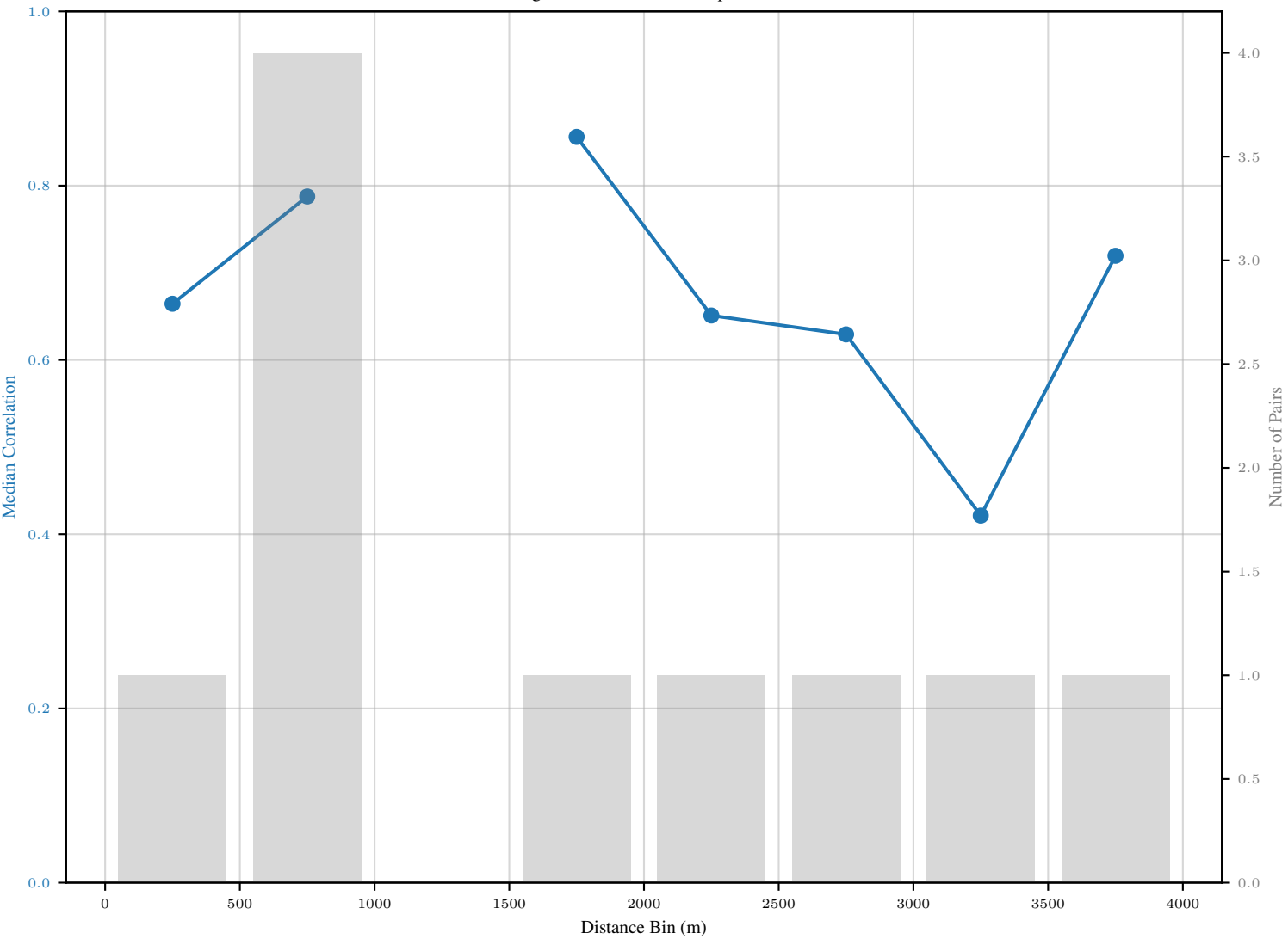
Stadt Tübingen: Median Correlation per Distance Bin
