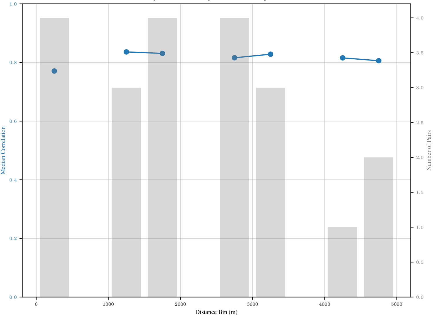
Ravensburg Tws Gmbh & Co. Kg: Median Correlation per Distance Bin
