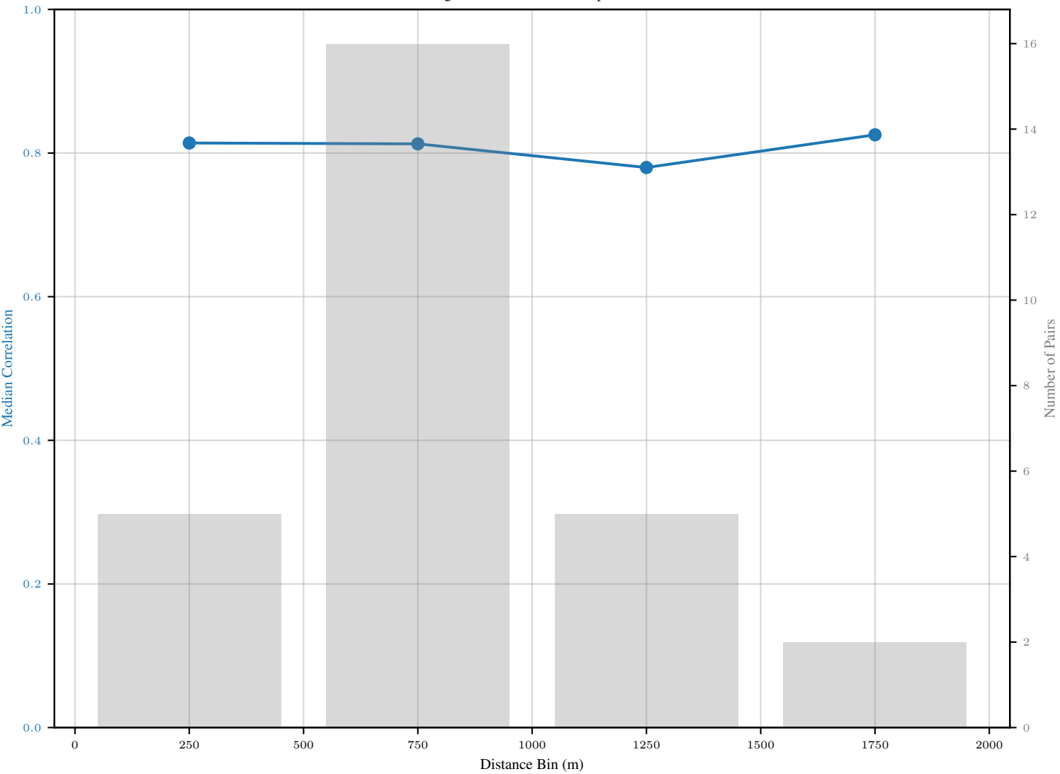
Stadt Reutlingen: Median Correlation per Distance Bin
