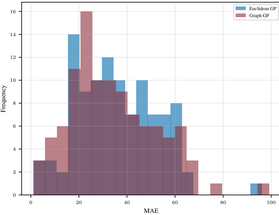
MAE Distribution
