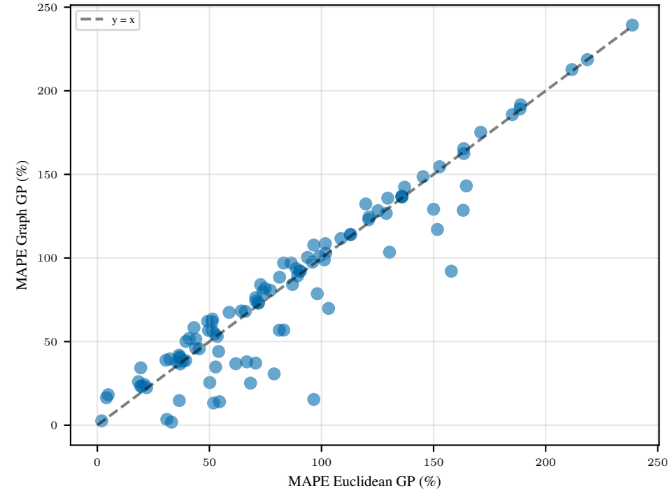
MAPE Comparison
