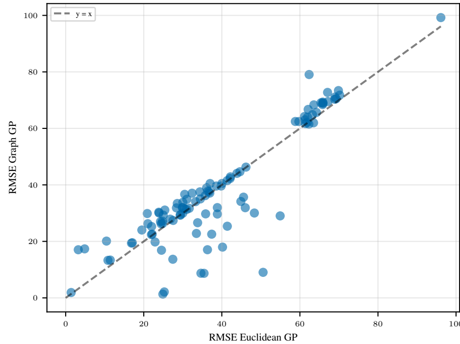
RMSE Comparison
