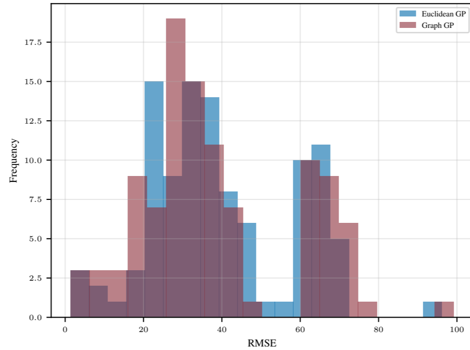
RMSE Distribution
