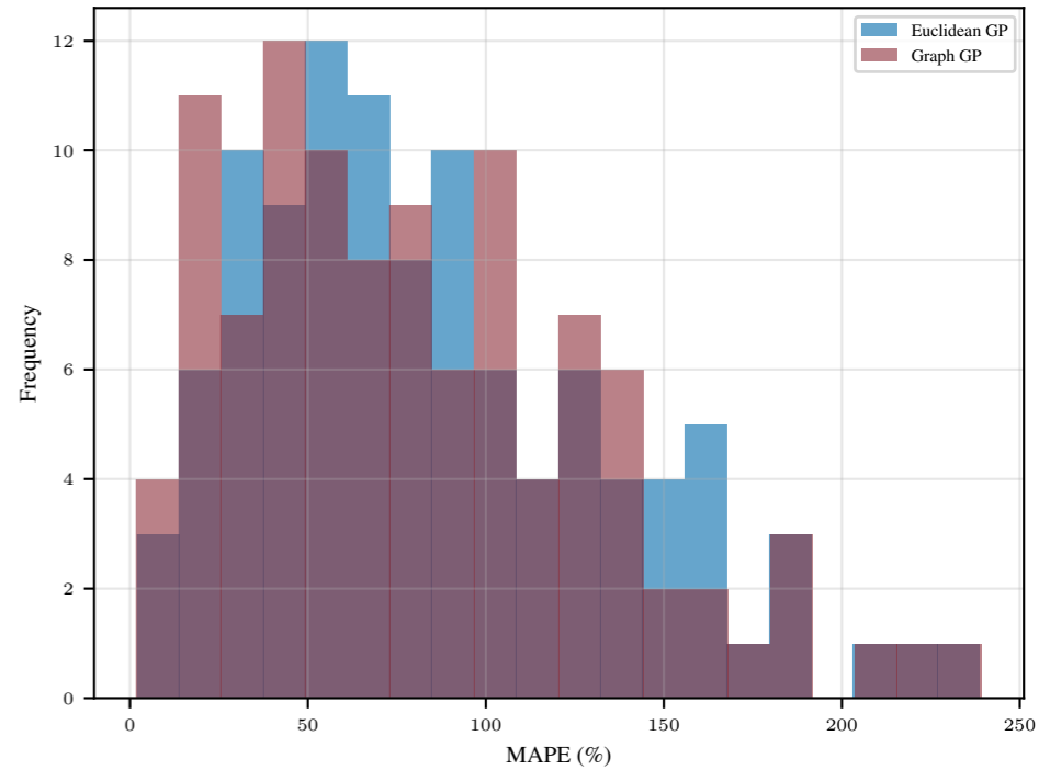
MAPE Distribution
