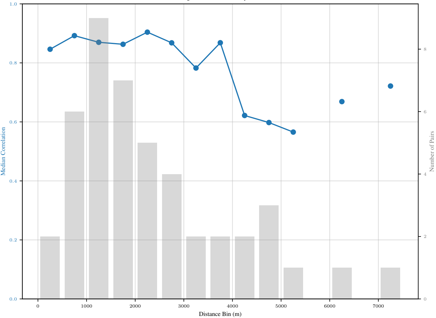
Stadt Freiburg: Median Correlation per Distance Bin
