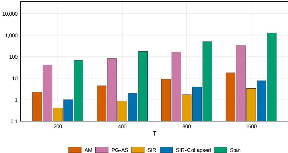
Total CPU time (hours)
