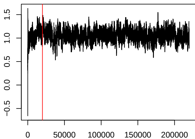
\theta_{1200,1}
