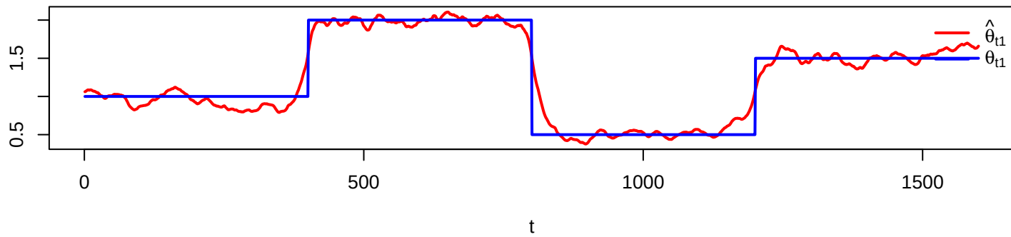
\theta_{t1} (chain 1)
