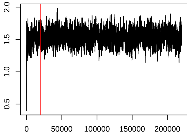
\theta_{400,1}
