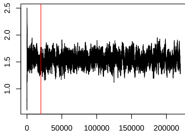
\theta_{800,1}
