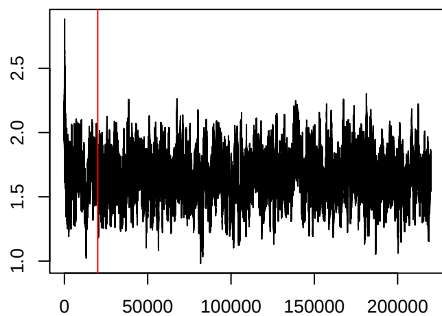
\theta_{1600,1}
