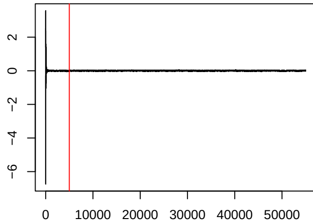
\theta_{1600,2}
