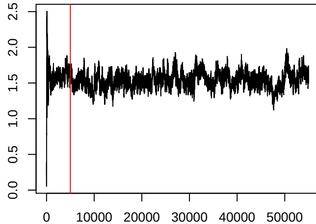
\theta_{800,1}
