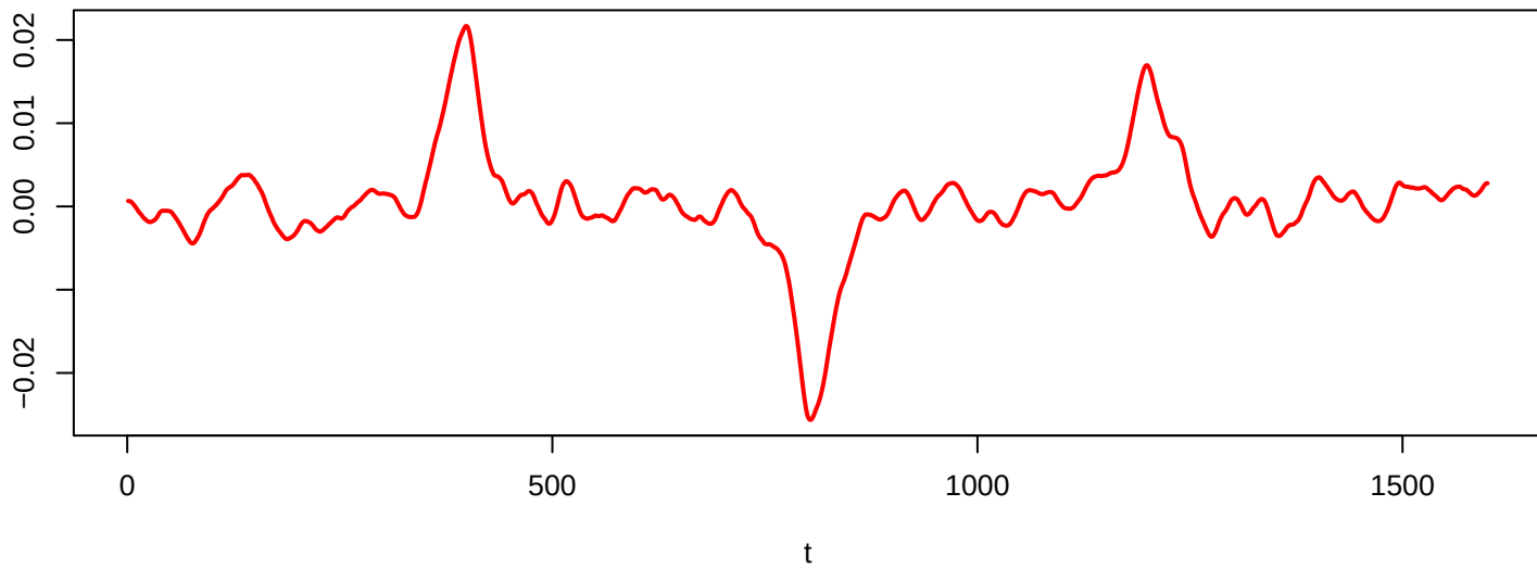
theta_t2 (chain 1)
