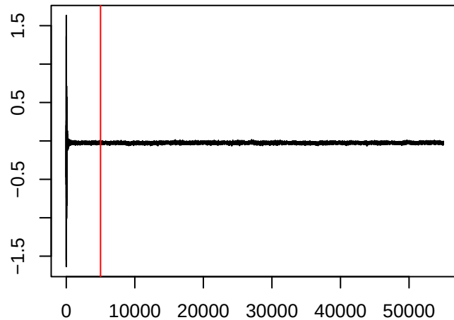
\theta_{800,2}
