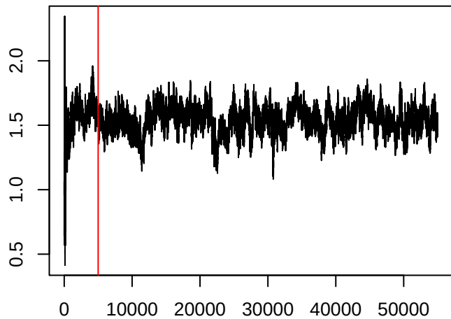
\theta_{400,1}
