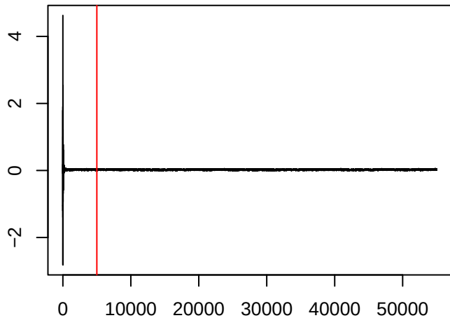
\theta_{400,2}
