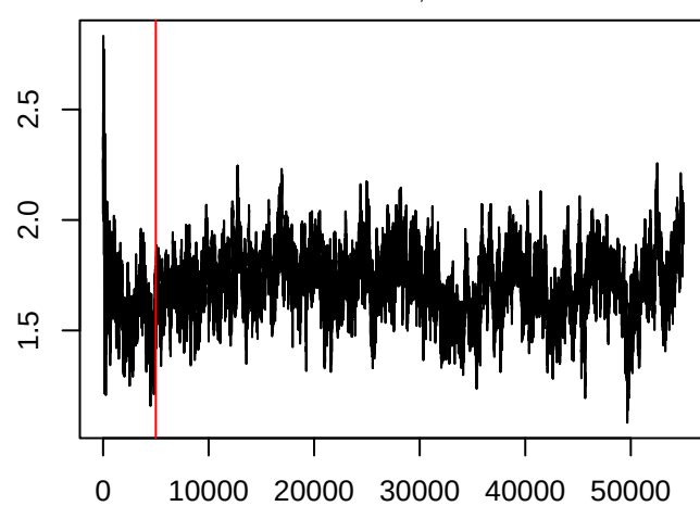
\theta_{1600,1}
