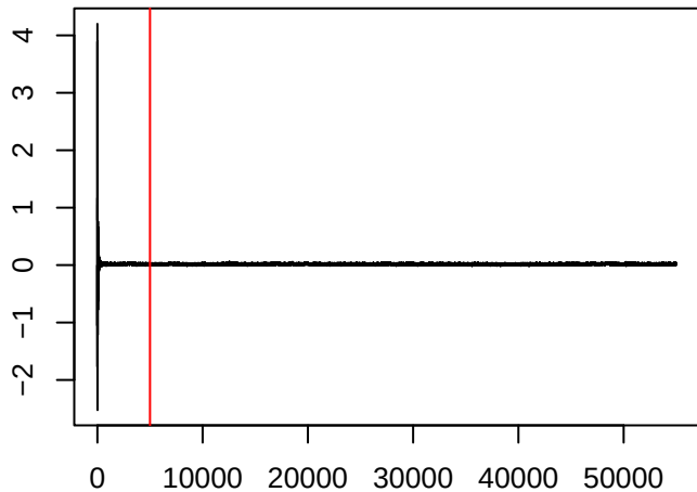
\theta_{1200,2}
