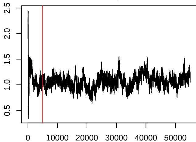
\theta_{1200,1}
