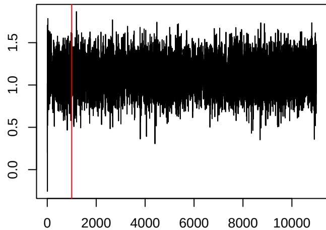
\theta_{150,1}
