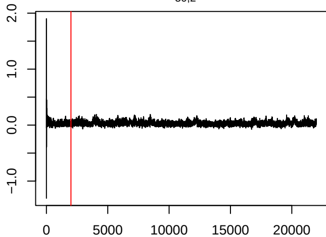
\theta_{50,2}
