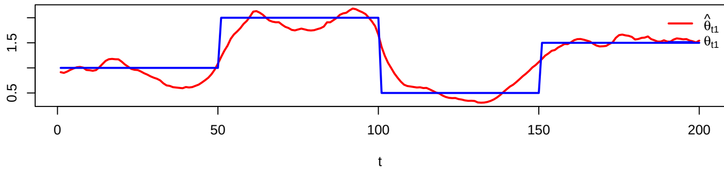
\theta_{t1} (chain 1)
