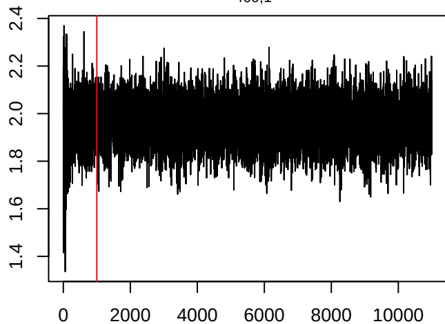
\theta_{400,1}
