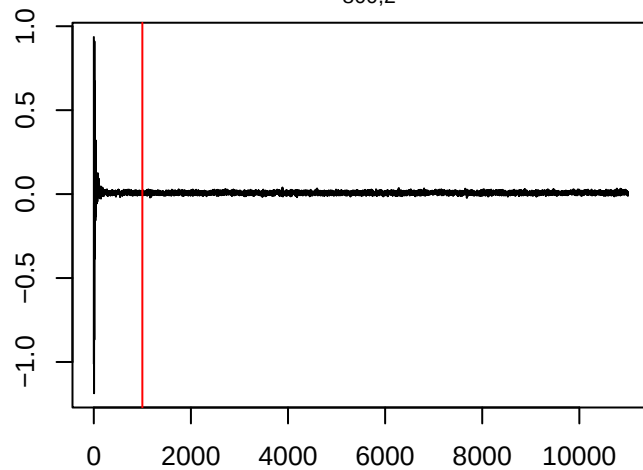
\theta_{800,2}
