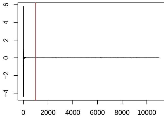
\theta_{1200,2}
