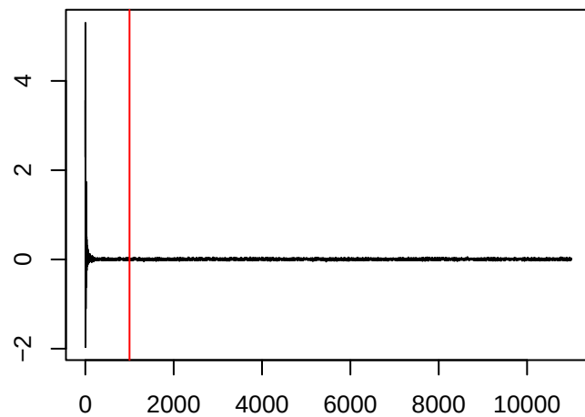
\theta_{1600,2}
