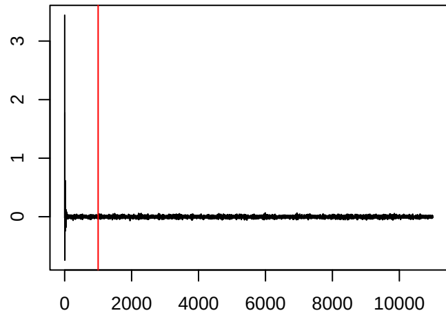
\theta_{175,2}
