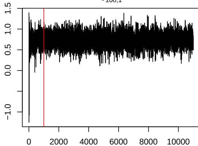
\theta_{100,1}
