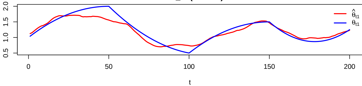
\theta_{t1} (chain 1)
