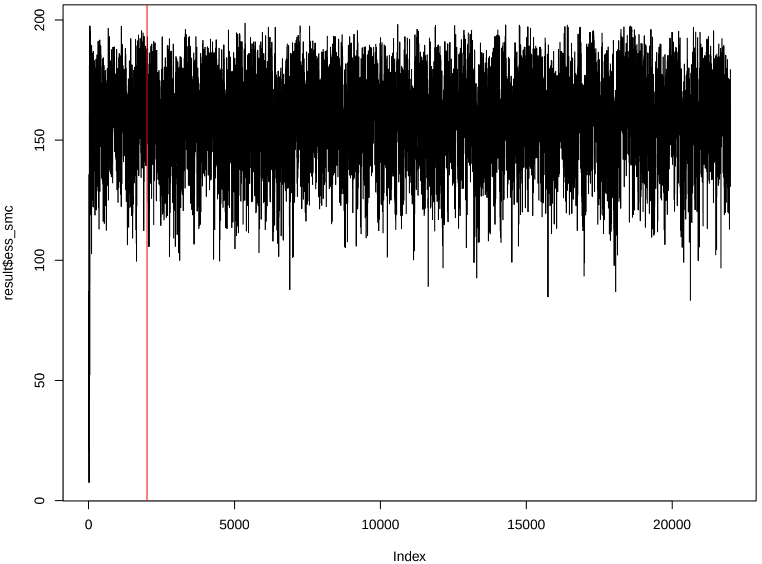
Effective Sample Size – SMC
