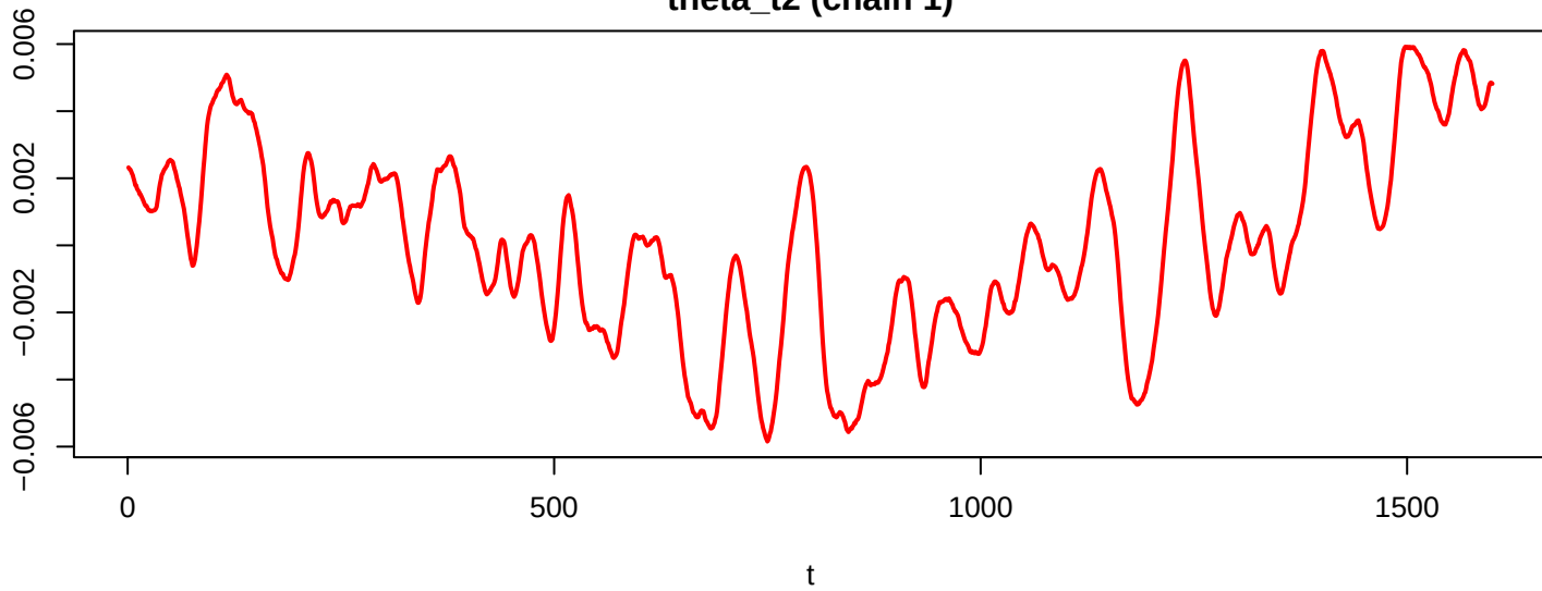
theta_t2 (chain 1)
