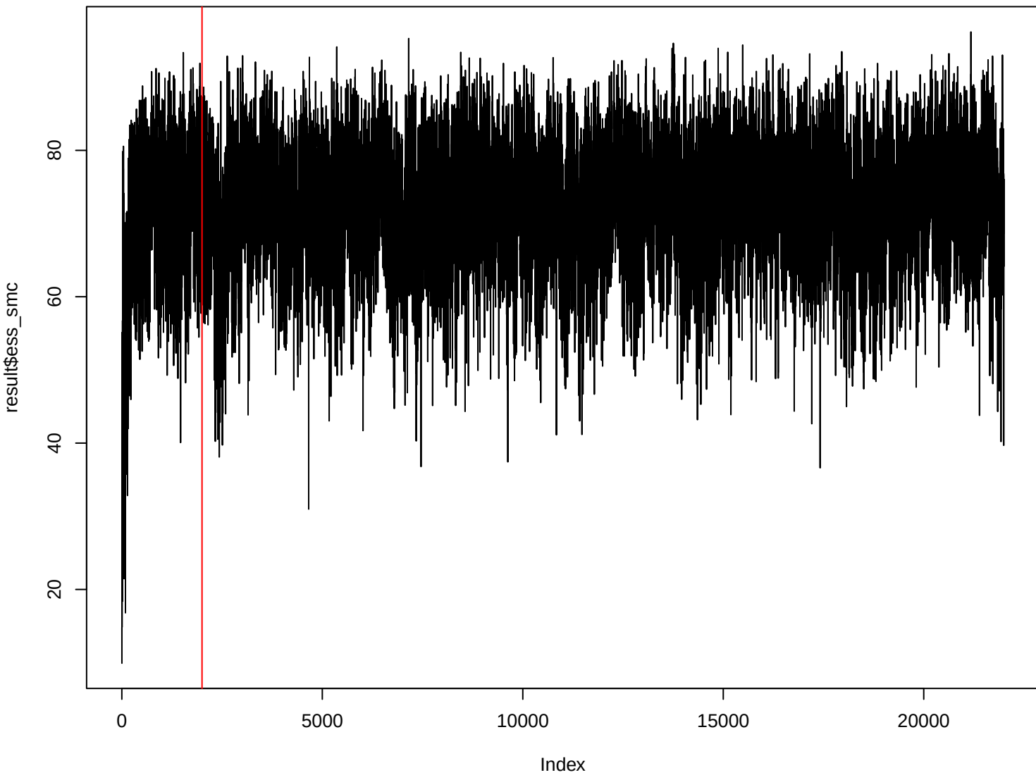
Effective Sample Size – SMC
