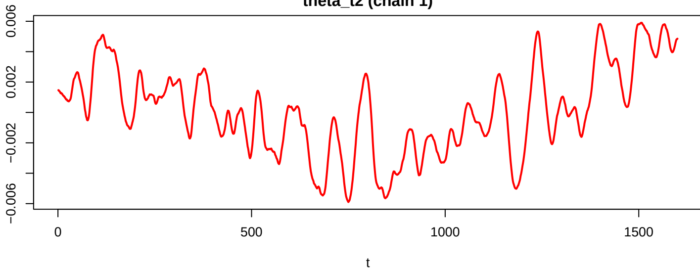
theta_t2 (chain 1)
