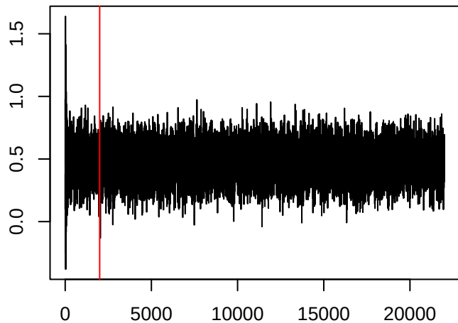
\theta_{1200,1}
