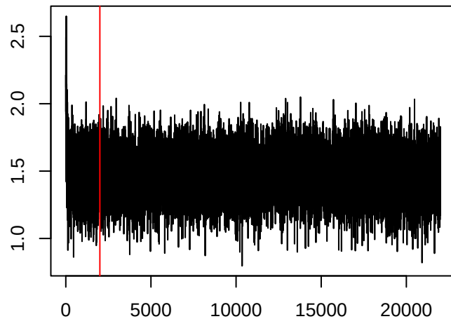
\theta_{1600,1}
