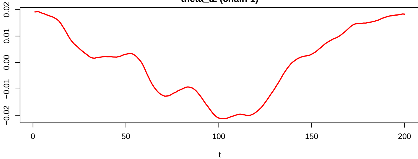
theta_t2 (chain 1)
