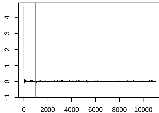
\theta_{175,2}
