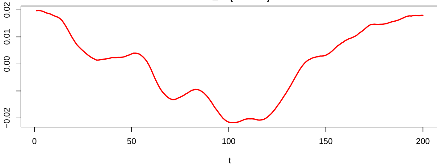
theta_t2 (chain 1)
