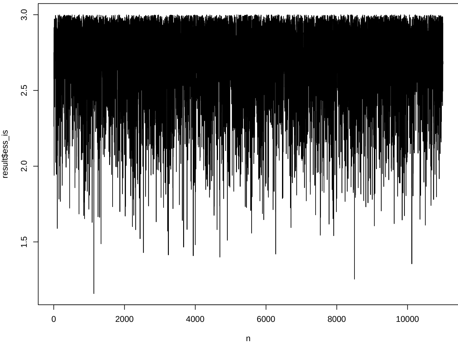
Effective Sample Size – IS
