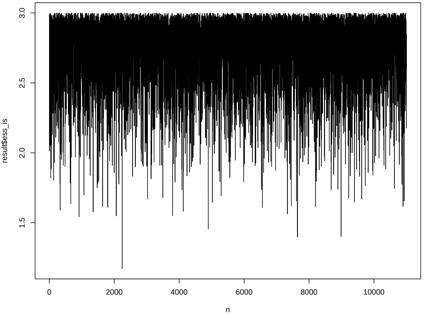
Effective Sample Size – IS
