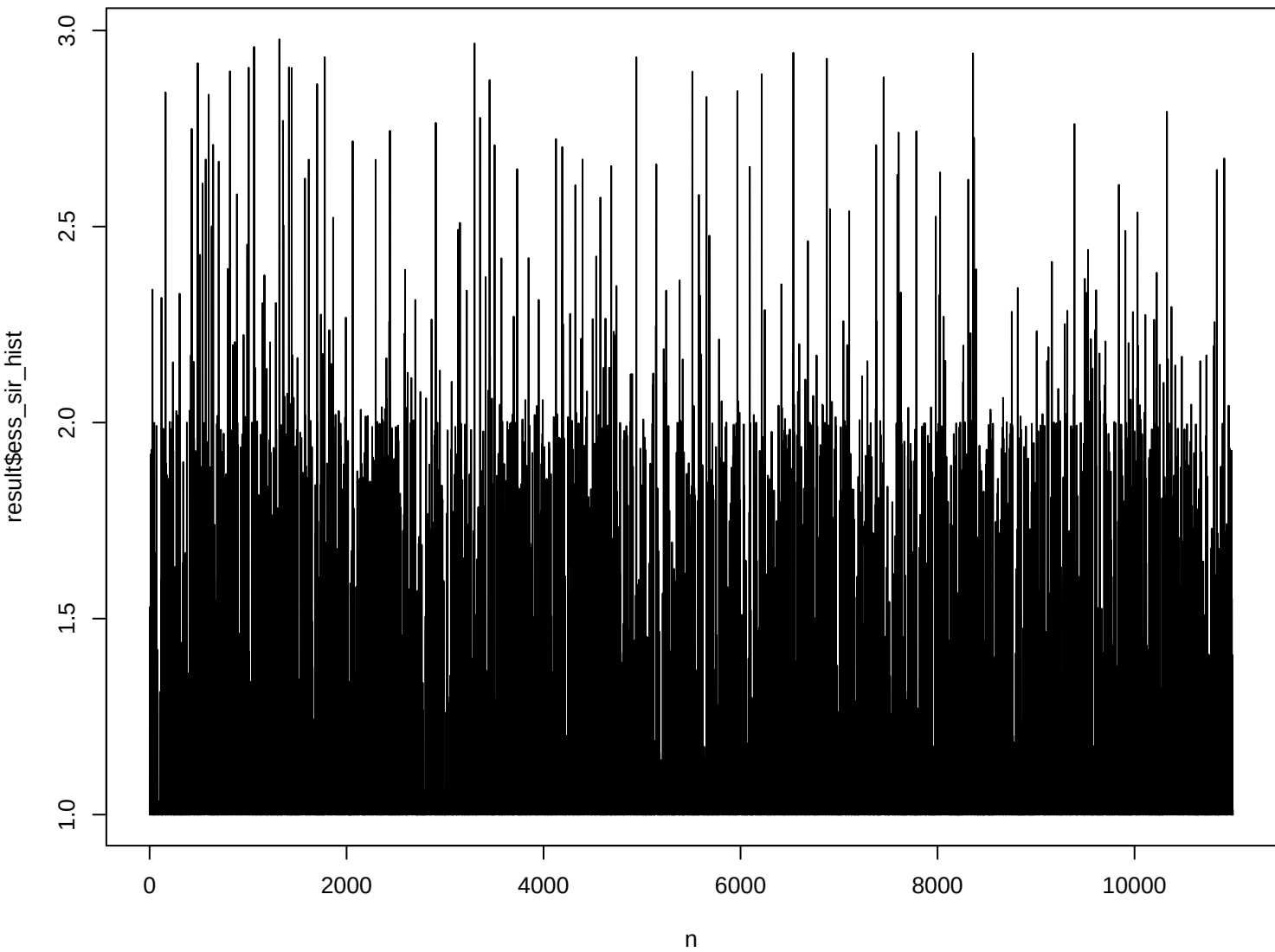
ESS - SIR theta1
