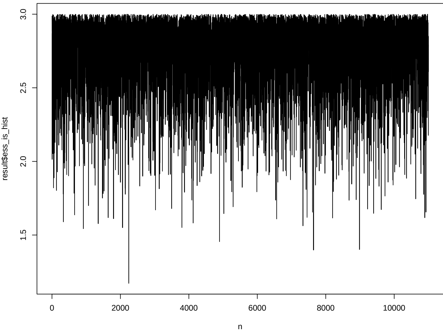
ESS – IS Integrated Likelihood (W1)
